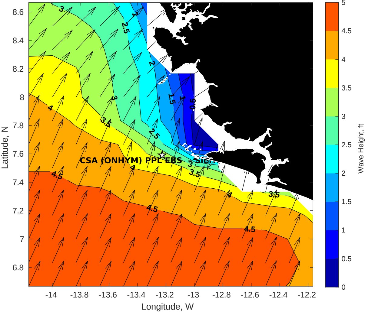
Wave Height (ft) for CSA (ONHYM) PPL EBS - Sierra Leone at 07-May-2025 09:00:00
