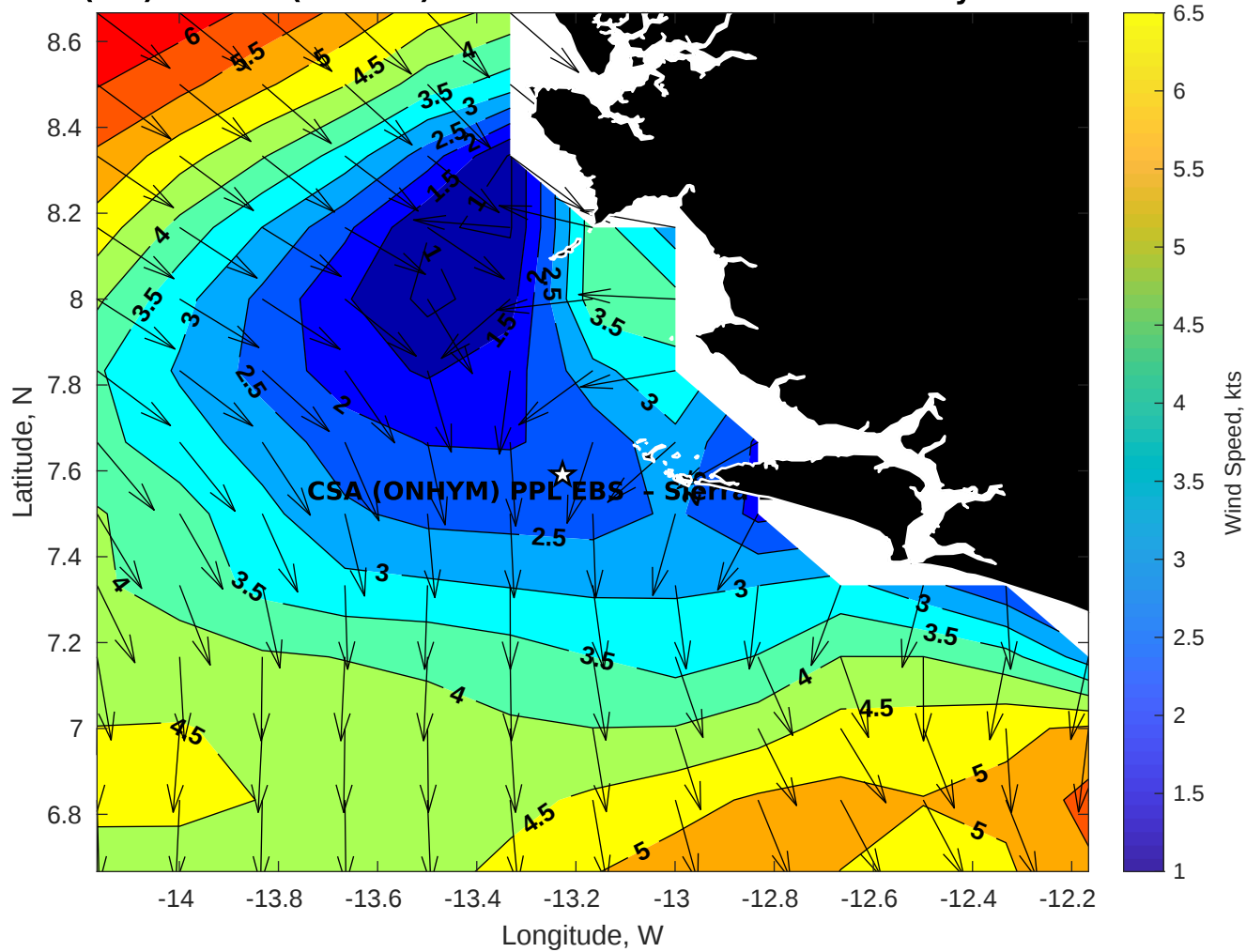
Winds (kts) for CSA (ONHYM) PPL EBS - Sierra Leone at 07-May-2025 09:00:00
