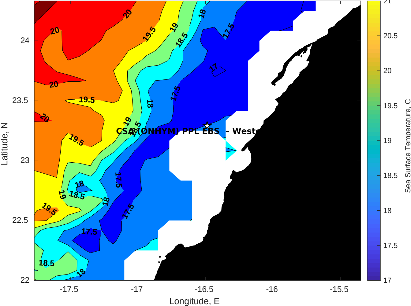
SST for CSA (ONHYM) PPL EBS - Western Sahara at 06-May-2025 00:00:00
