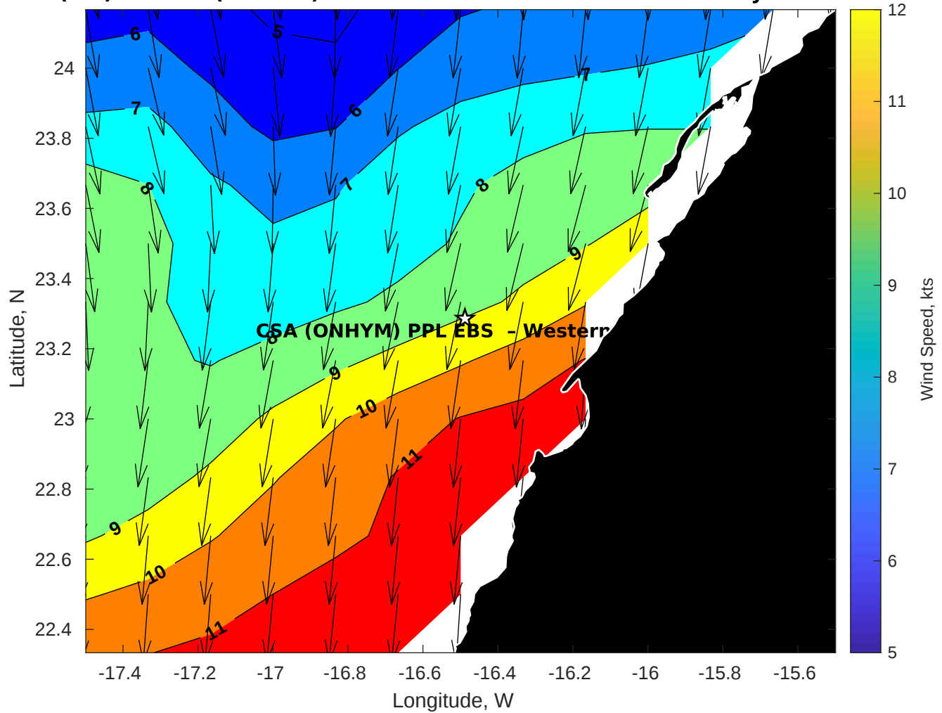
Winds (kts) for CSA (ONHYM) PPL EBS - Western Sahara at 07-May-2025 09:00:00
