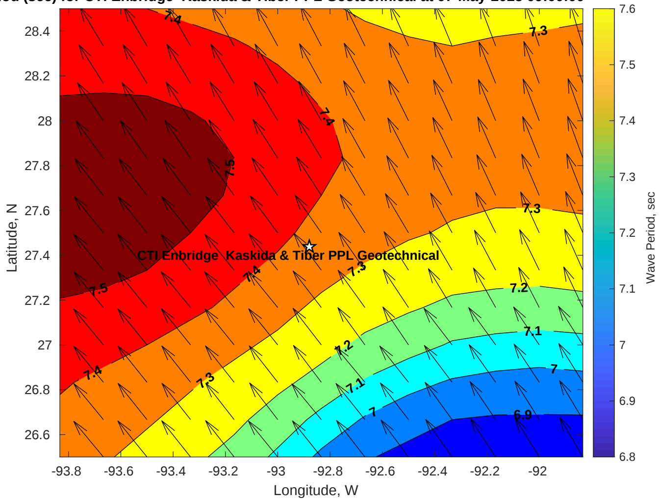
Wave Period (sec) for CTI Enbridge Kaskida & Tiber PPL Geotechnical at 07-May-2025 09:00:00
