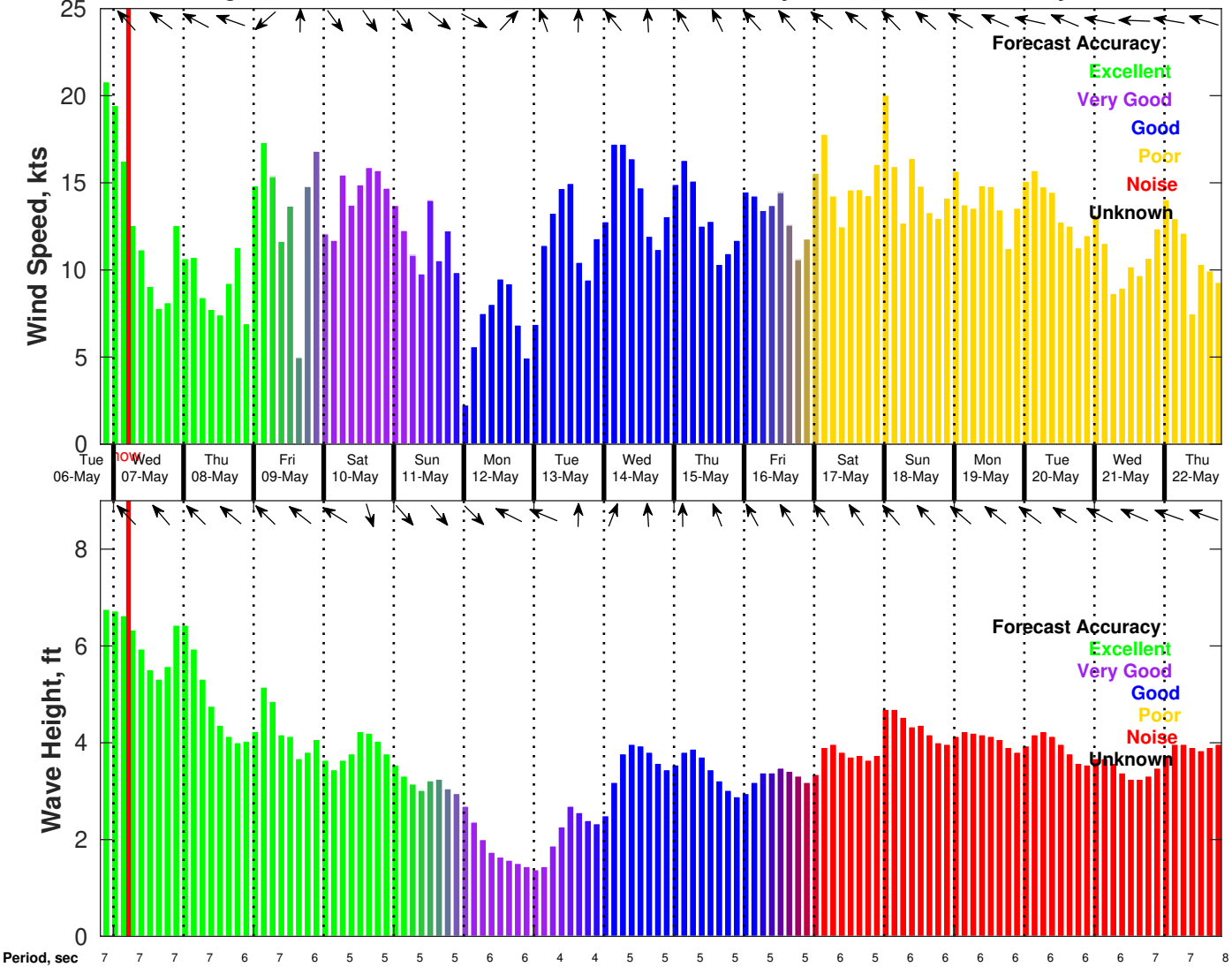
Wind & Wave Forecast for CTI Enbridge Kaskida & Tiber PPL Geotechnical from 06-May-2025 20:00:00 to 22-May-2025 20:00:00
