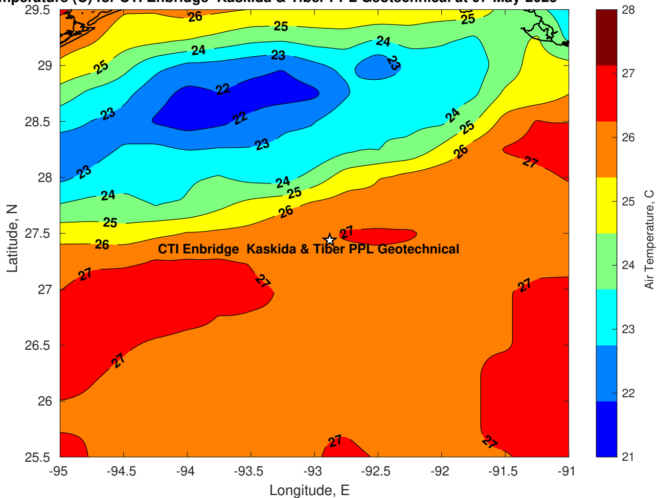
Air Temperature (C) for CTI Enbridge Kaskida & Tiber PPL Geotechnical at 07-May-2025
