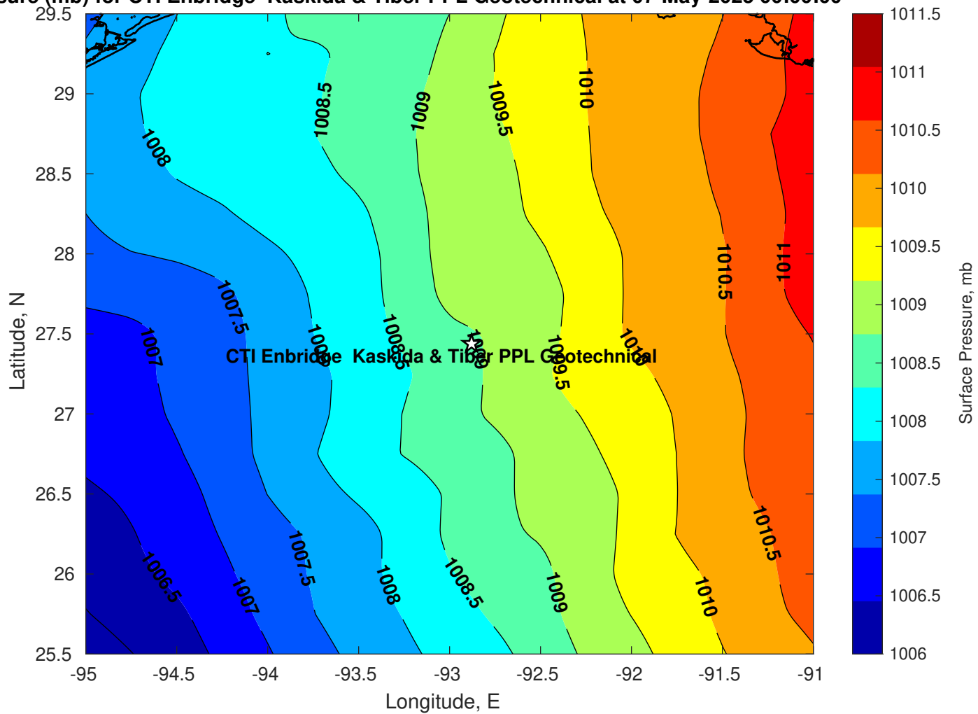
Surface Pressure (mb) for CTI Enbridge Kaskida & Tiber PPL Geotechnical at 07-May-2025 00:00:00
