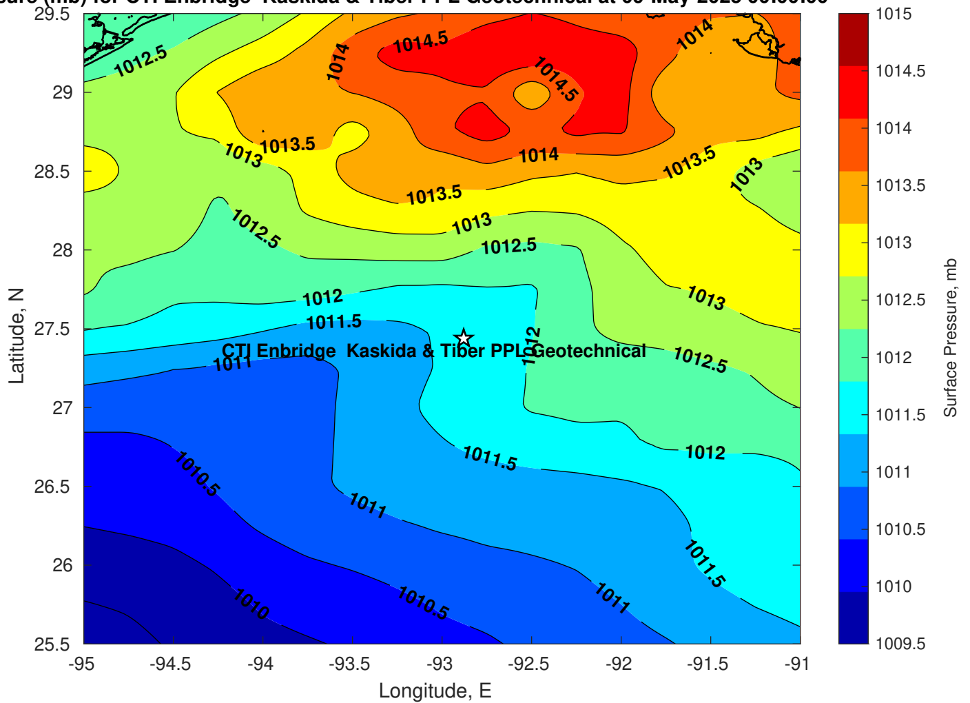
Surface Pressure (mb) for CTI Enbridge Kaskida & Tiber PPL Geotechnical at 09-May-2025 00:00:00
