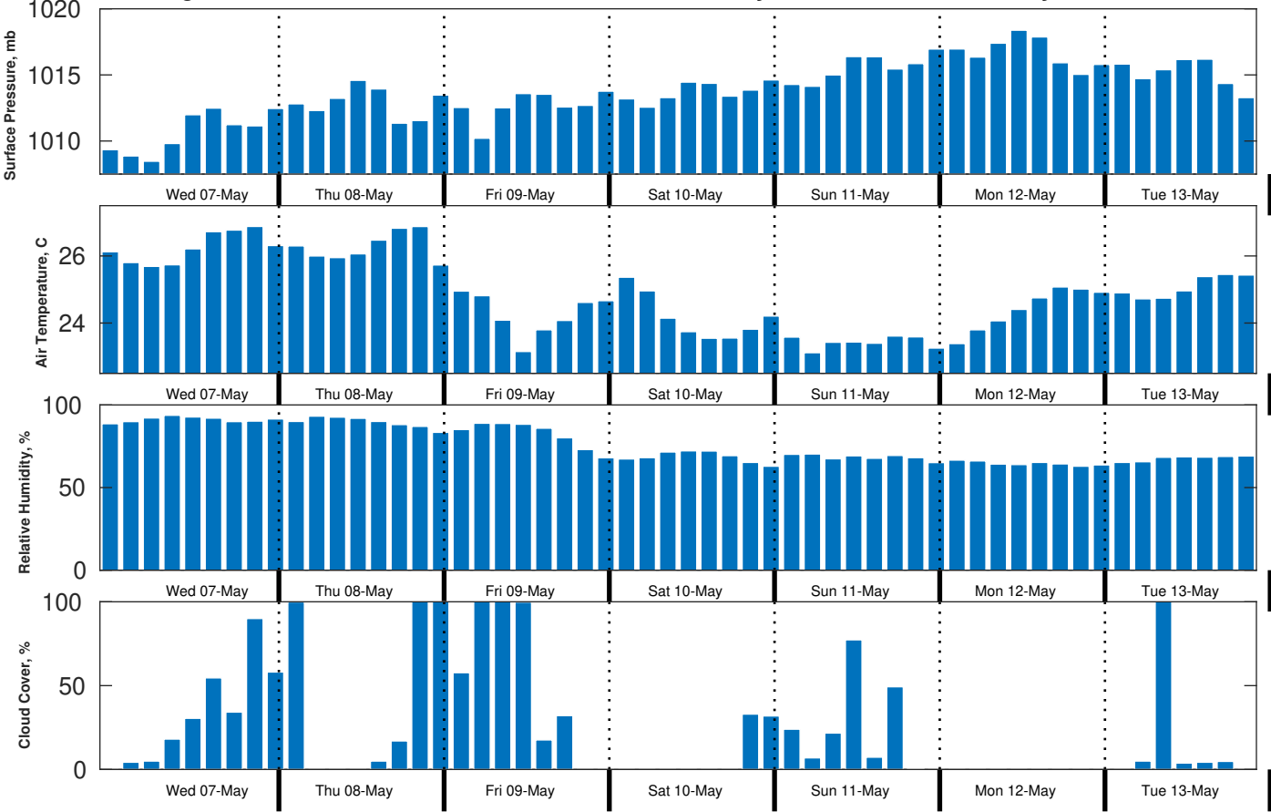
Met Forecast for CTI Enbridge Kaskida & Tiber PPL Geotechnical from 07-May-2025 00:00:00 to 14-May-2025 00:00:00
