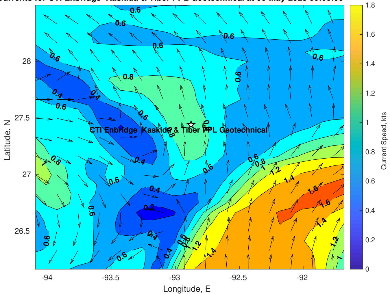
Surface Currents for CTI Enbridge Kaskida & Tiber PPL Geotechnical at 06-May-2025 00:00:00
