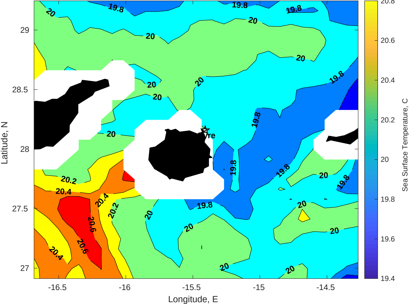
SST for Gyre at 06-May-2025 00:00:00
