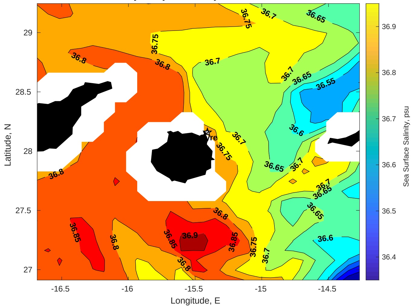
Surface Salinity for Gyre at 06-May-2025 00:00:00
