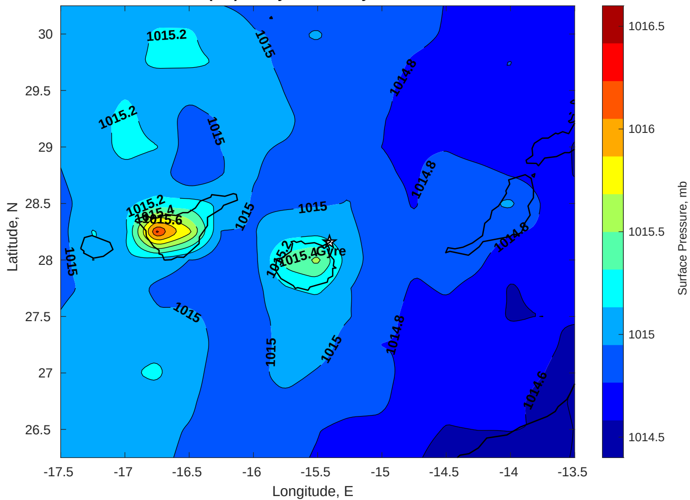
Surface Pressure (mb) for Gyre at 09-May-2025 00:00:00
