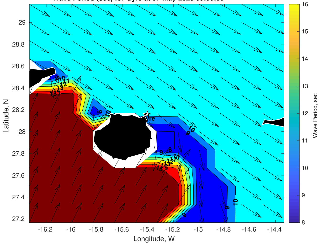
Wave Period (sec) for Gyre at 07-May-2025 09:00:00
