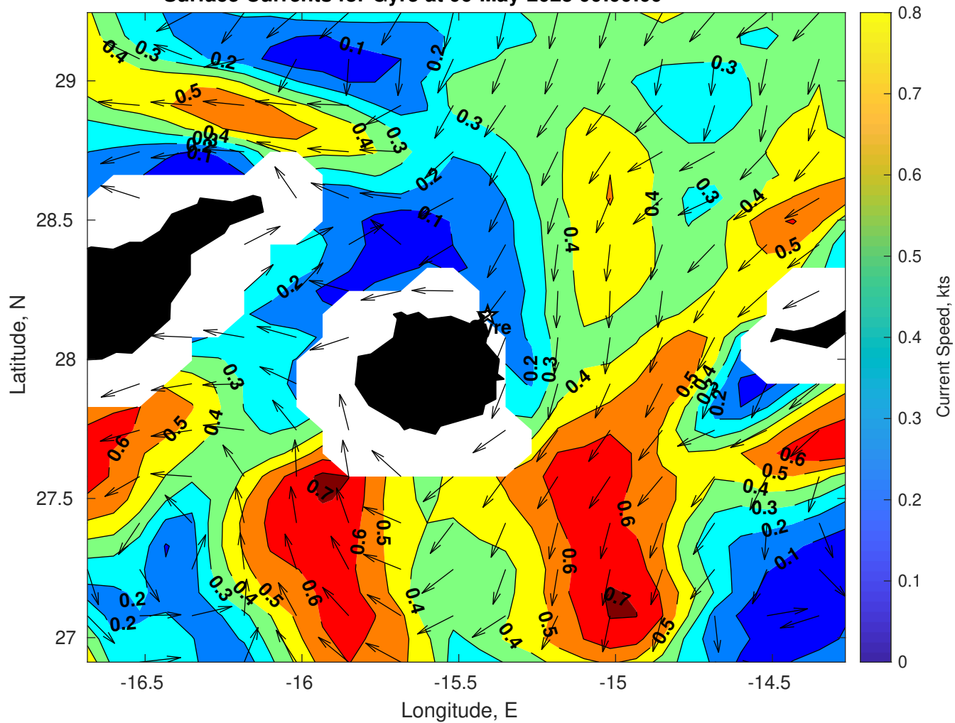
Surface Currents for Gyre at 06-May-2025 00:00:00
