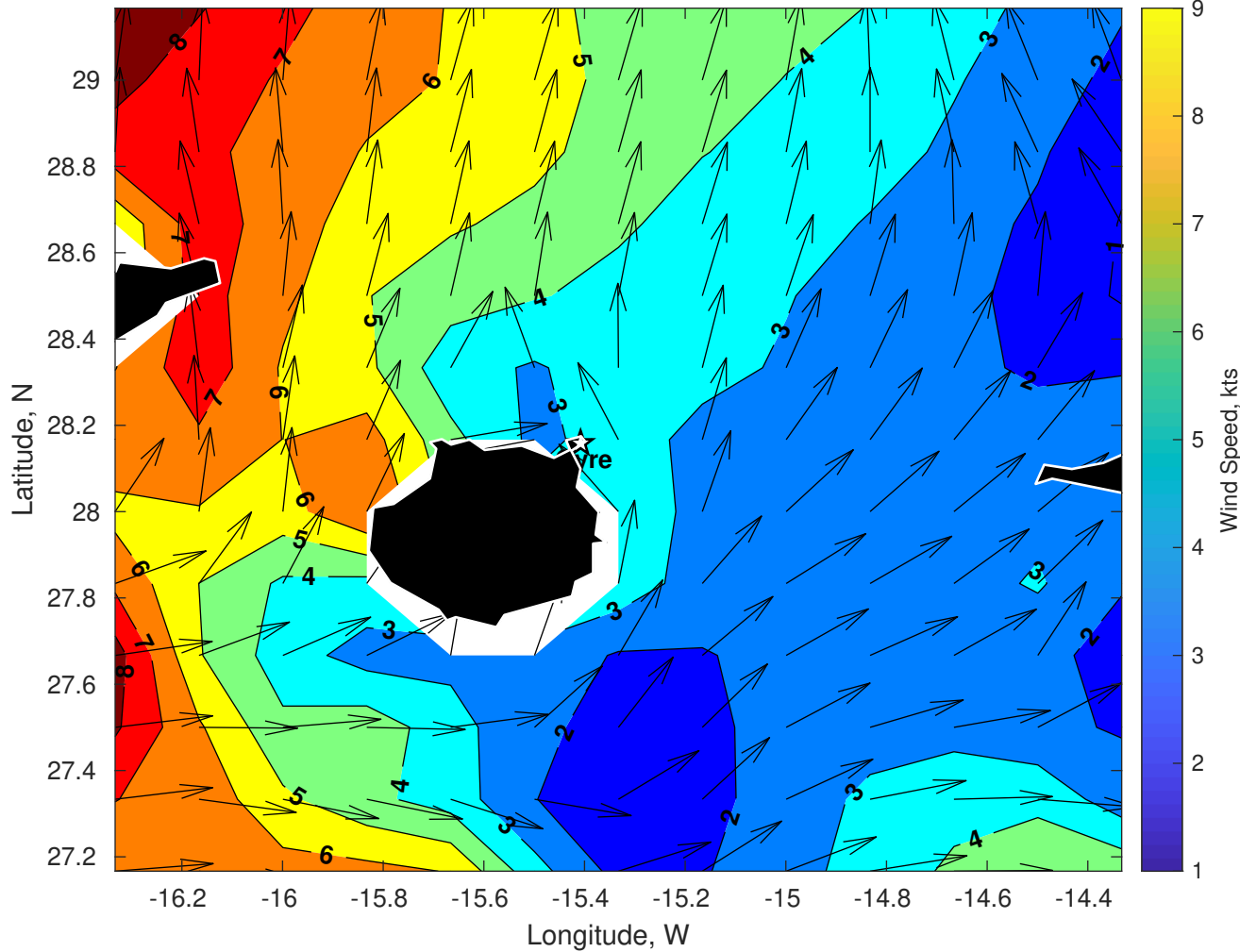
Winds (kts) for Gyre at 07-May-2025 09:00:00
