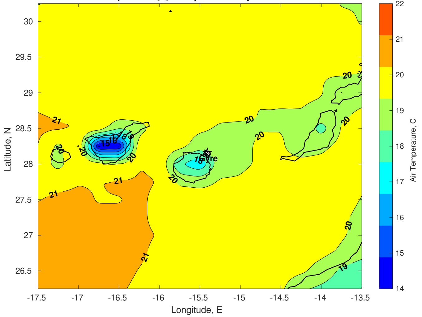
Air Temperature (C) for Gyre at 07-May-2025
