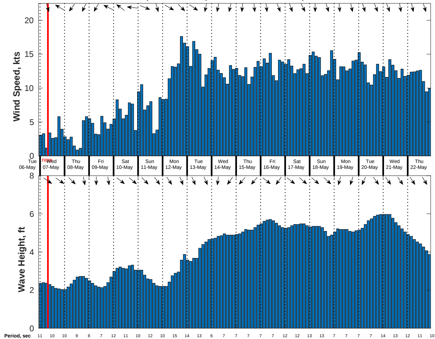
Wind & Wave Forecast for Gyre from 06-May-2025 23:00:00 to 22-May-2025 23:00:00
