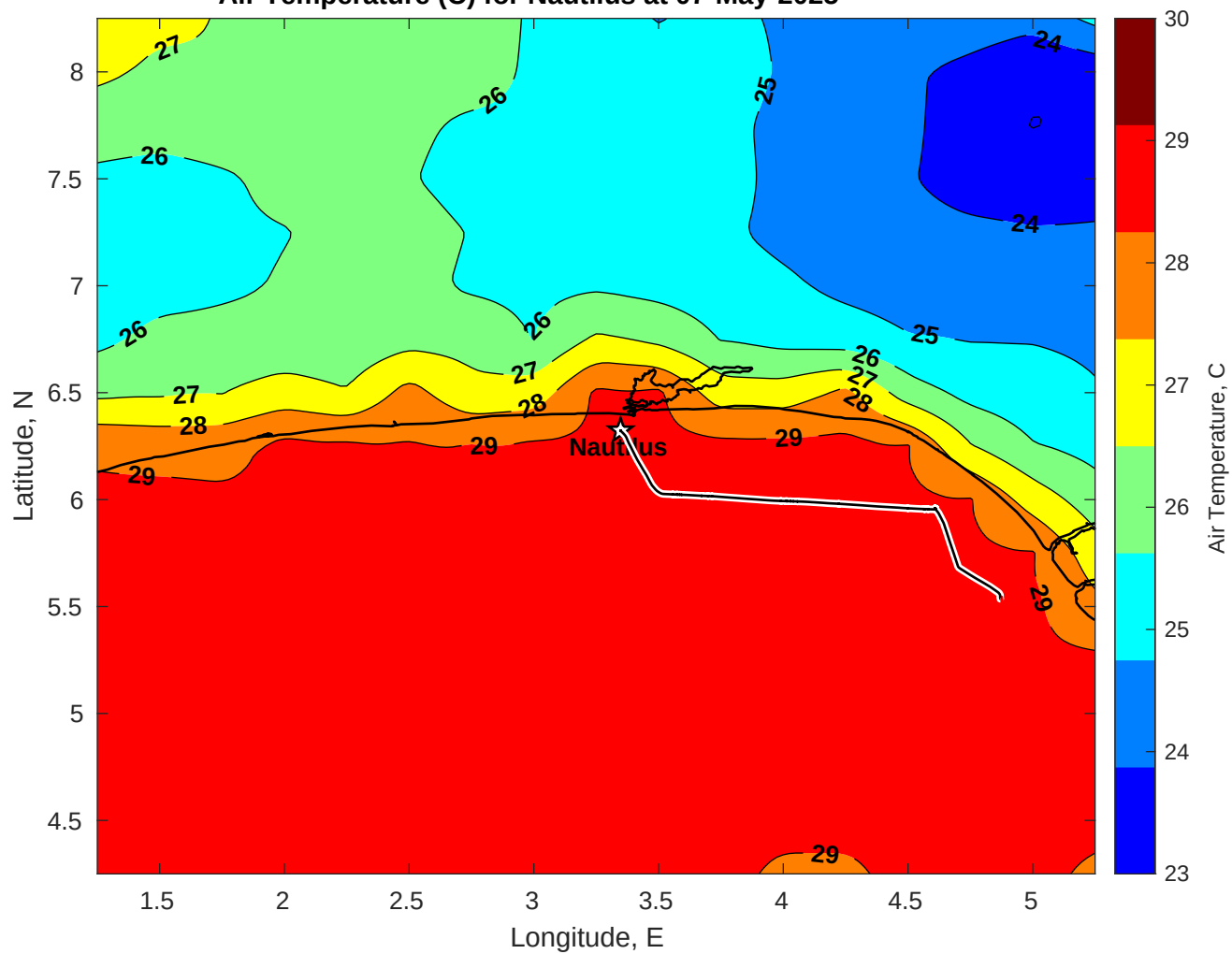
Air Temperature (C) for Nautilus at 07-May-2025
