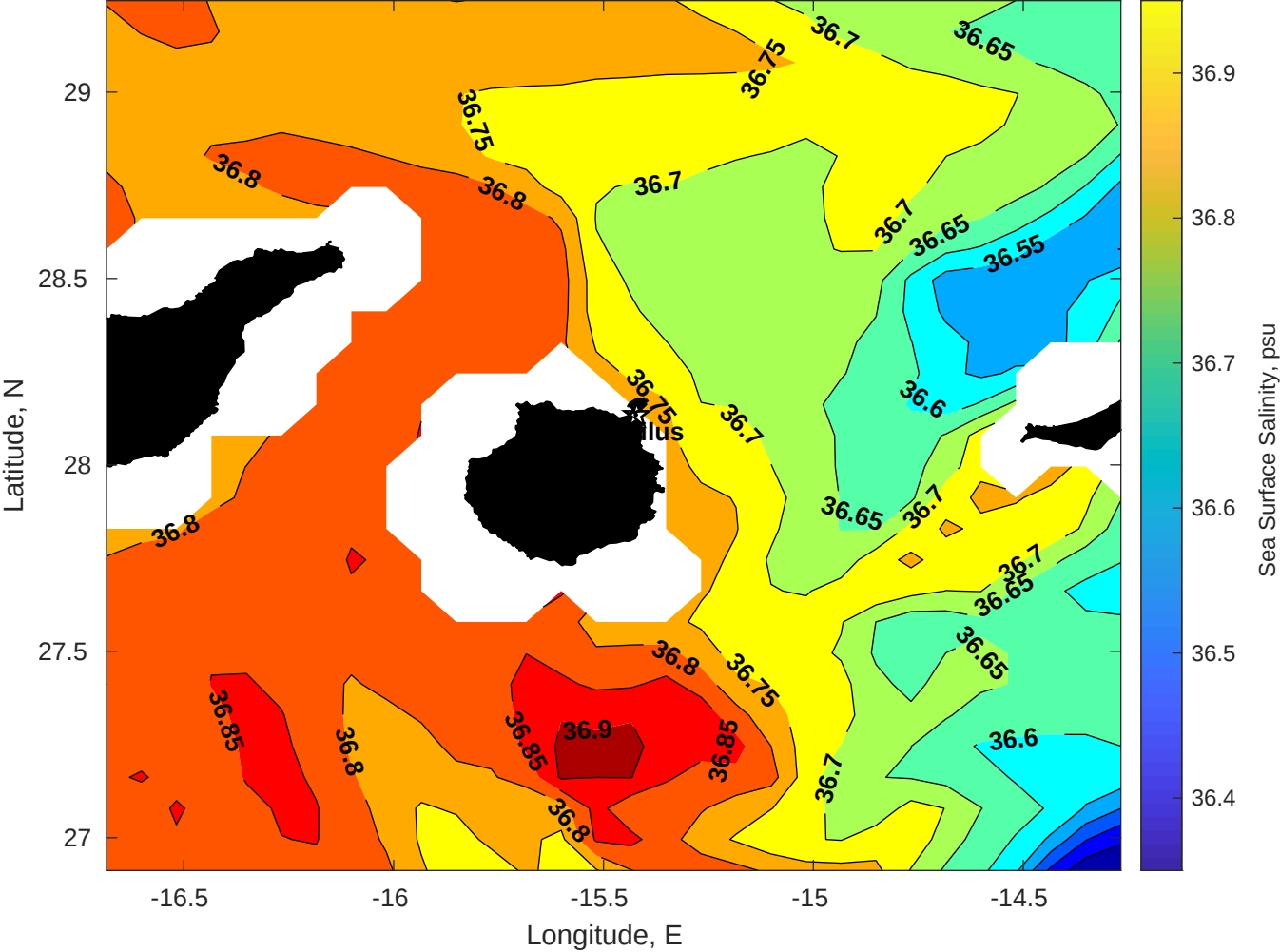
Surface Salinity for Nautilus at 06-May-2025 00:00:00
