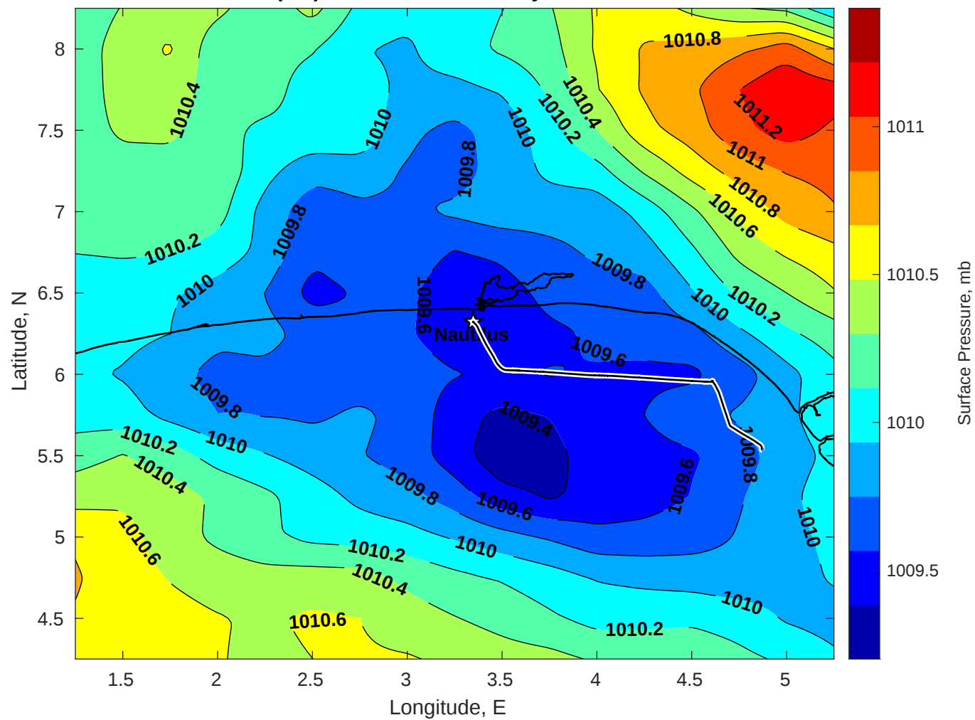
Surface Pressure (mb) for Nautilus at 08-May-2025 00:00:00
