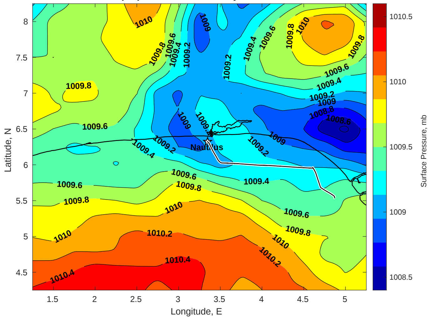
Surface Pressure (mb) for Nautilus at 09-May-2025 00:00:00
