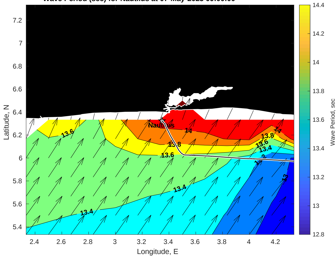
Wave Period (sec) for Nautilus at 07-May-2025 09:00:00
