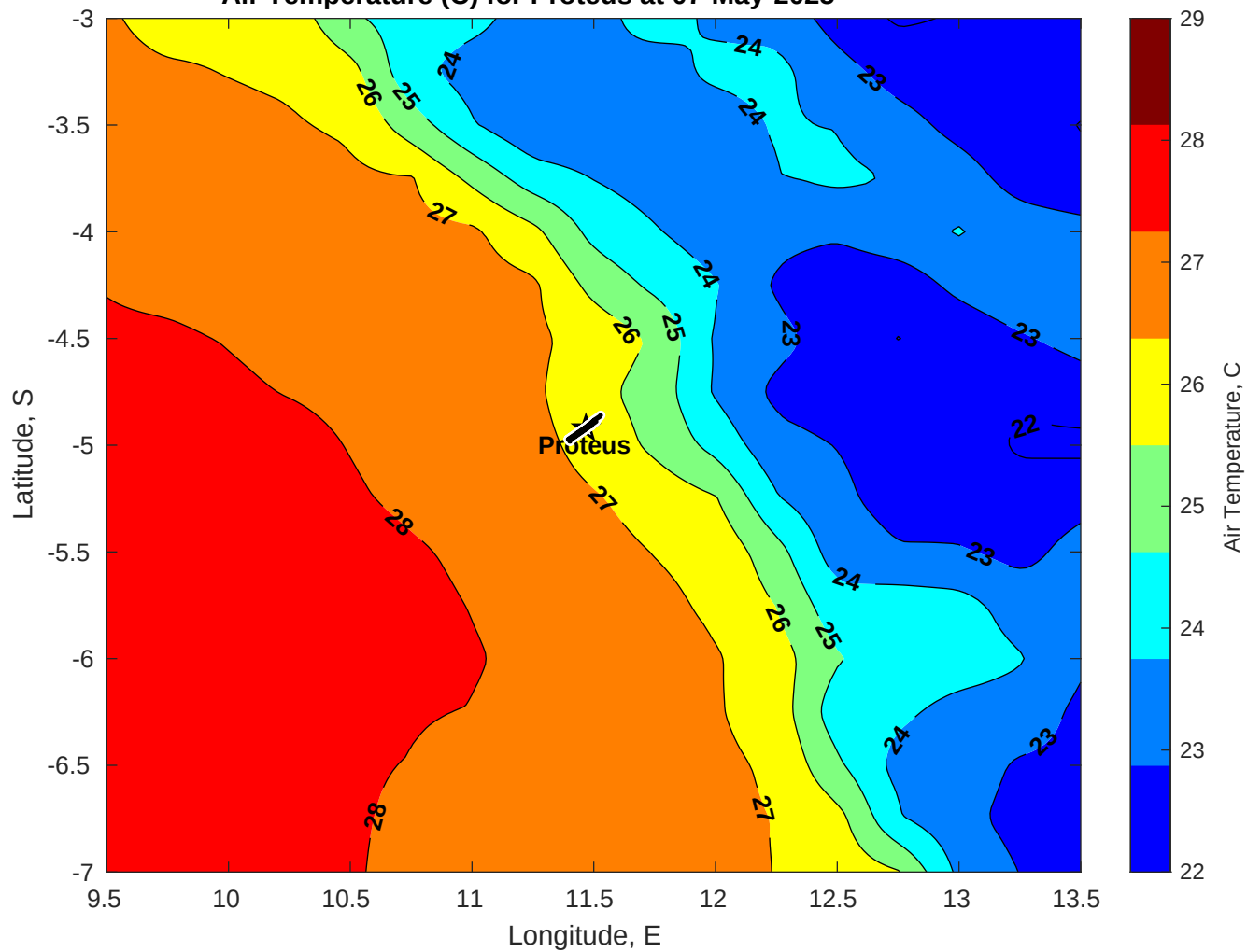
Air Temperature (C) for Proteus at 07-May-2025
