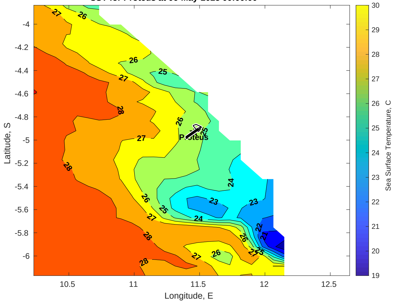
SST for Proteus at 06-May-2025 00:00:00
