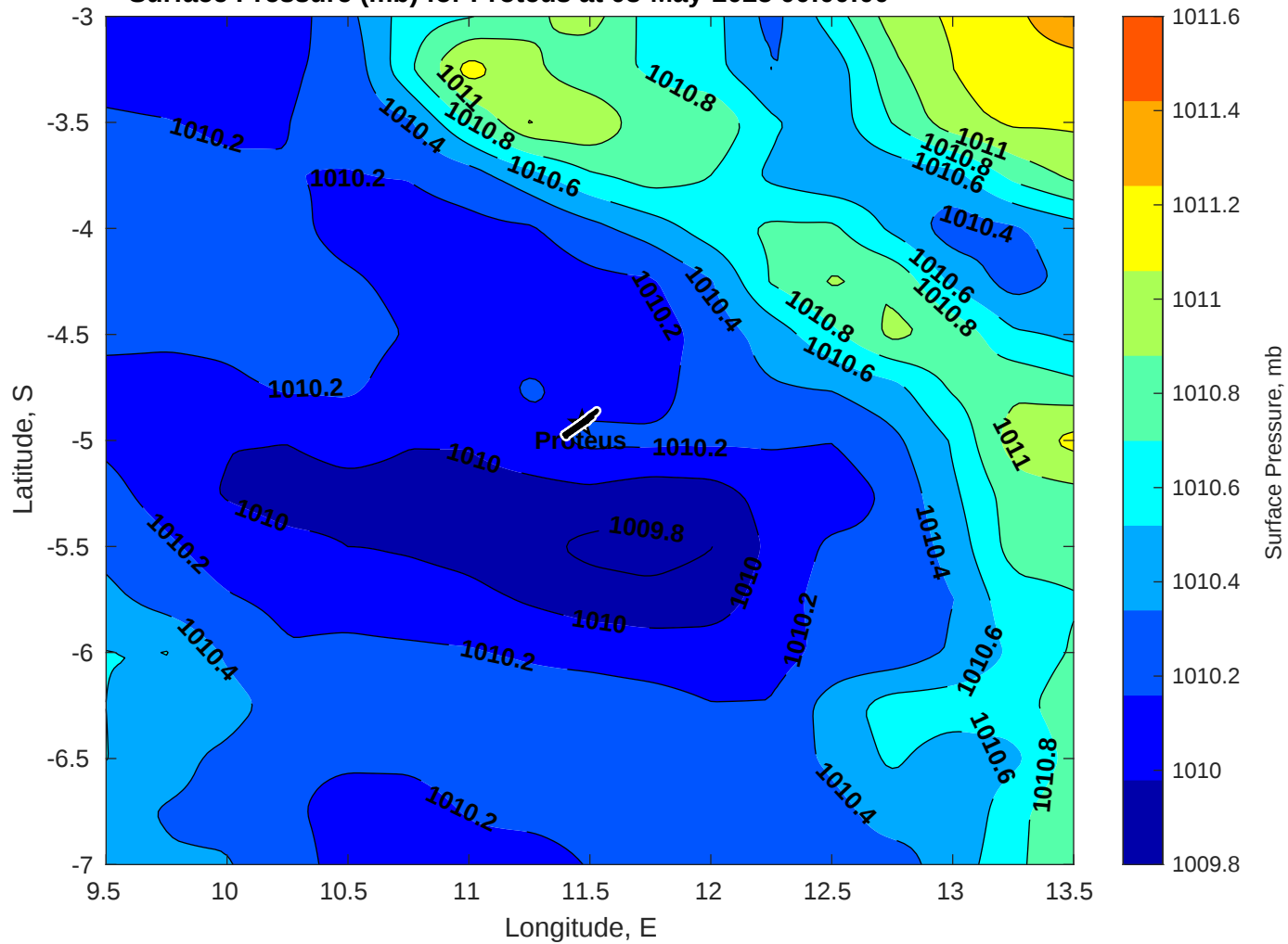
Surface Pressure (mb) for Proteus at 08-May-2025 00:00:00
