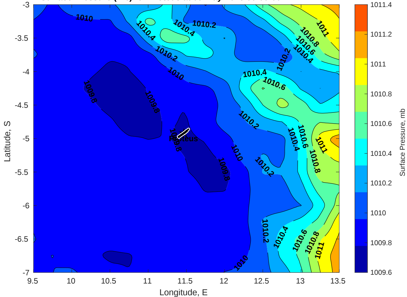
Surface Pressure (mb) for Proteus at 09-May-2025 00:00:00
