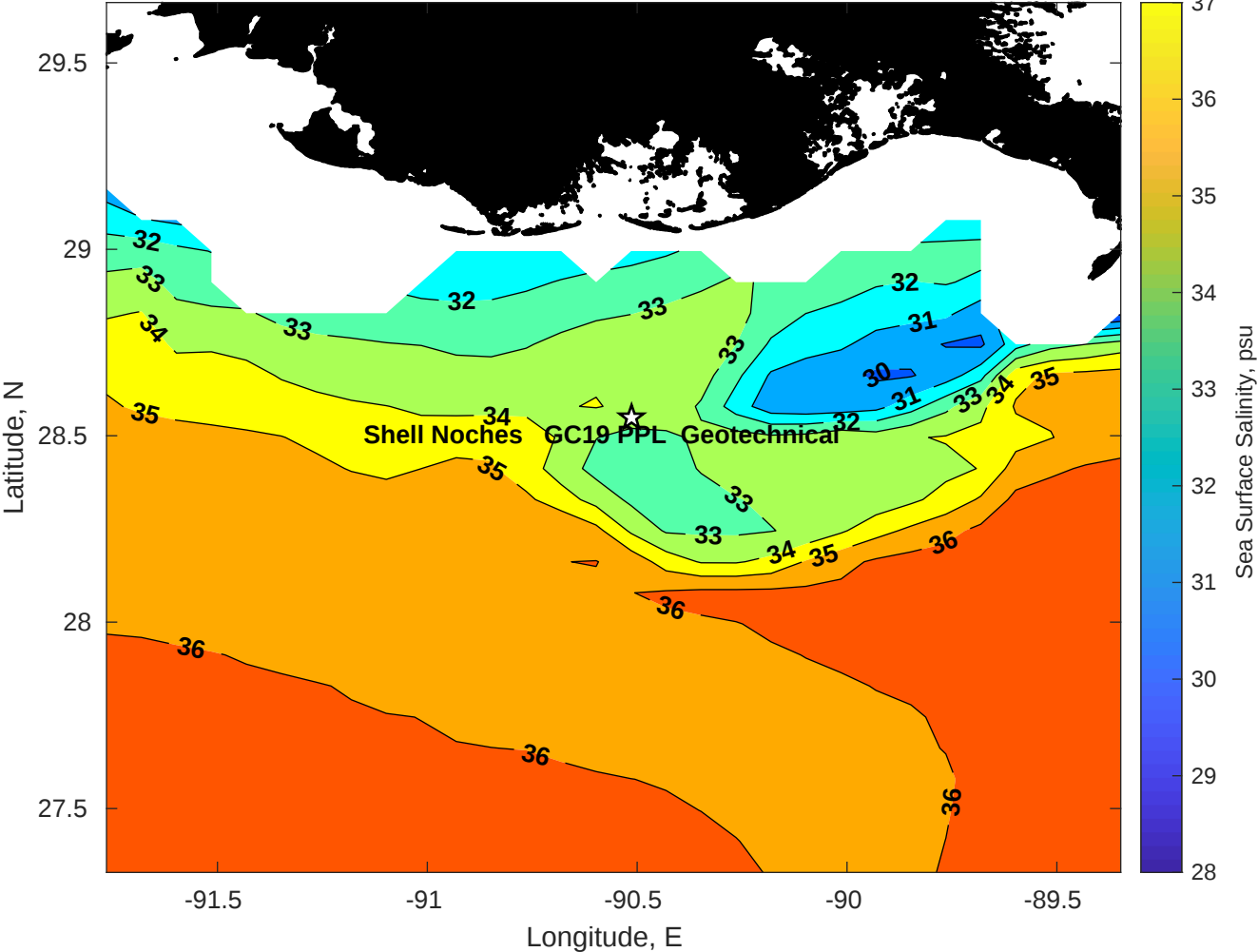
Surface Salinity for Shell Noches GC19 PPL Geotechnical at 06-May-2025 00:00:00
