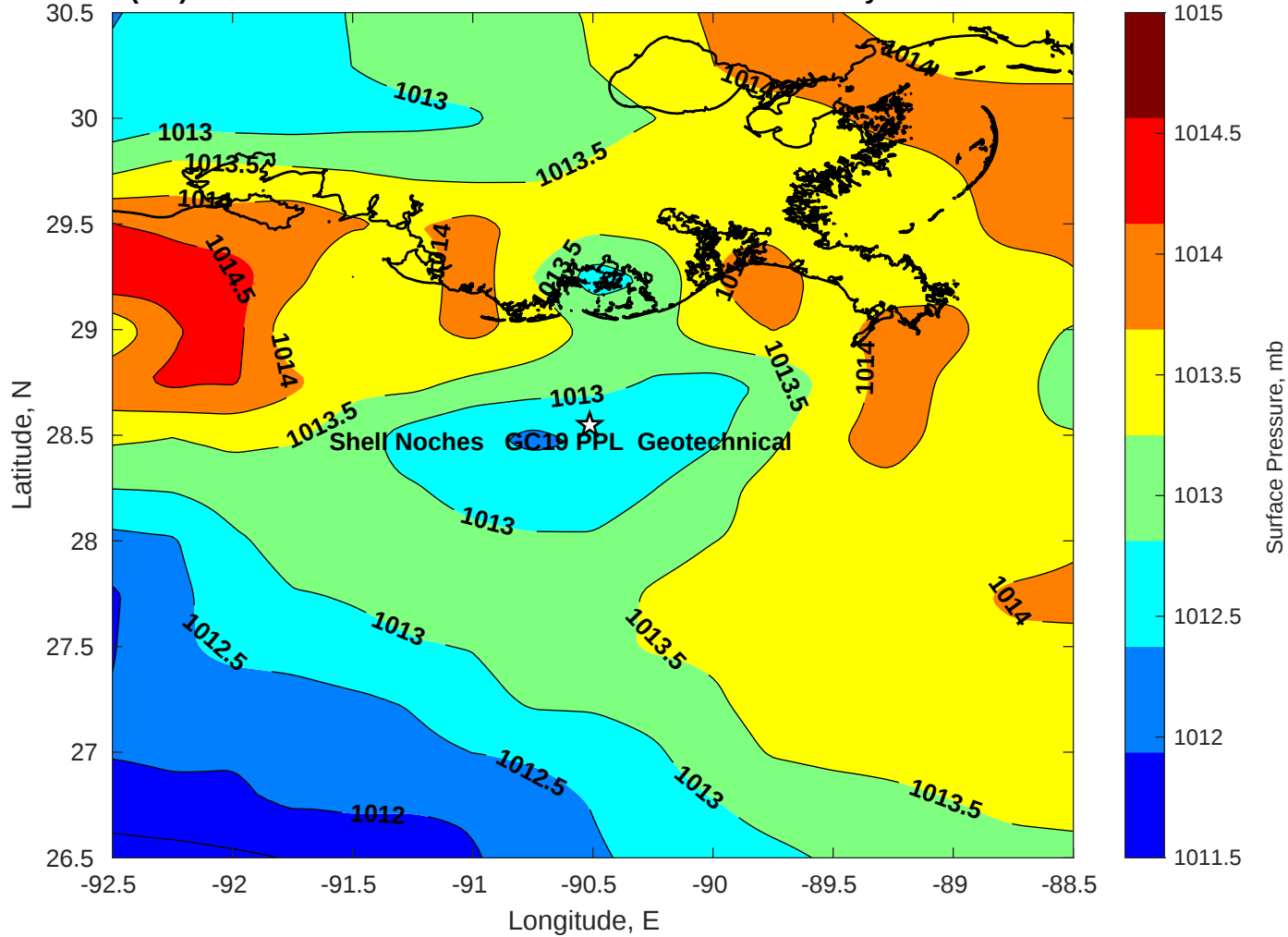
Surface Pressure (mb) for Shell Noches GC19 PPL Geotechnical at 09-May-2025 00:00:00
