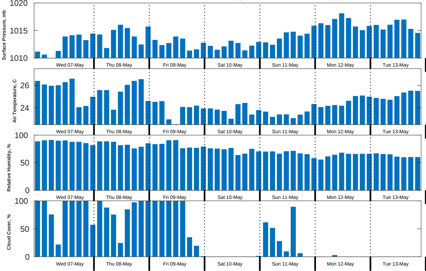
Met Forecast for Shell Noches GC19 PPL Geotechnical from 07-May-2025 00:00:00 to 14-May-2025 00:00:00
