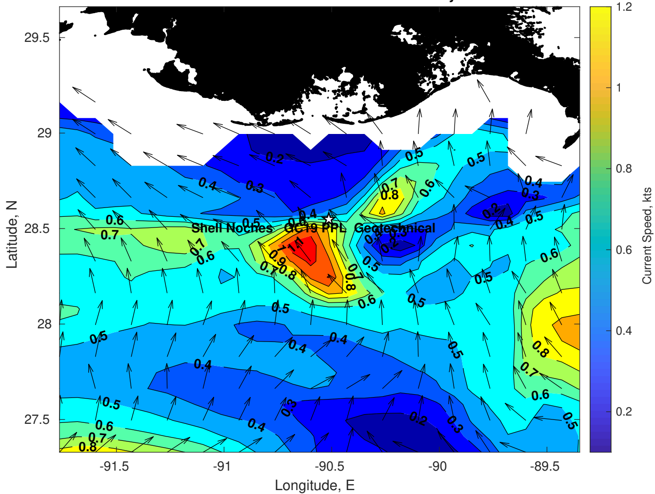
Surface Currents for Shell Noches GC19 PPL Geotechnical at 06-May-2025 00:00:00
