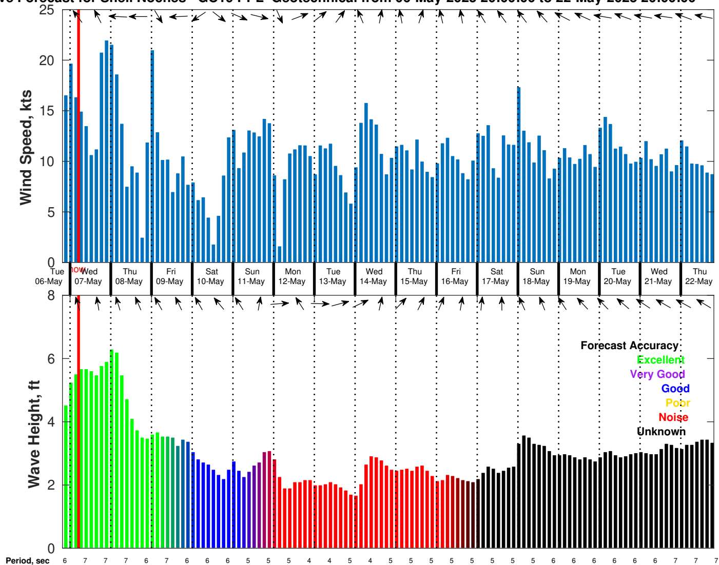
Wind & Wave Forecast for Shell Noches GC19 PPL Geotechnical from 06-May-2025 20:00:00 to 22-May-2025 20:00:00
