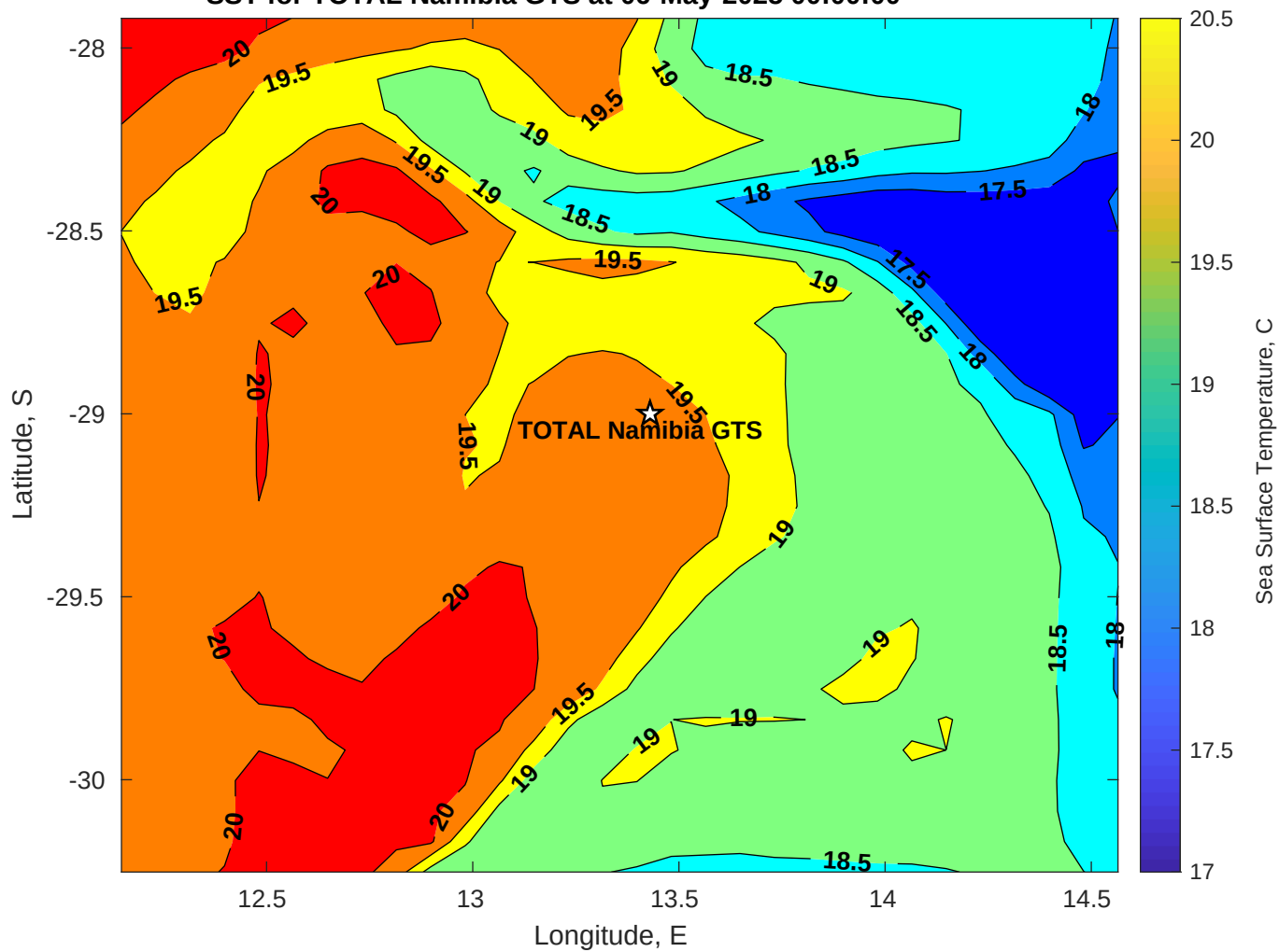
SST for TOTAL Namibia GTS at 06-May-2025 00:00:00
