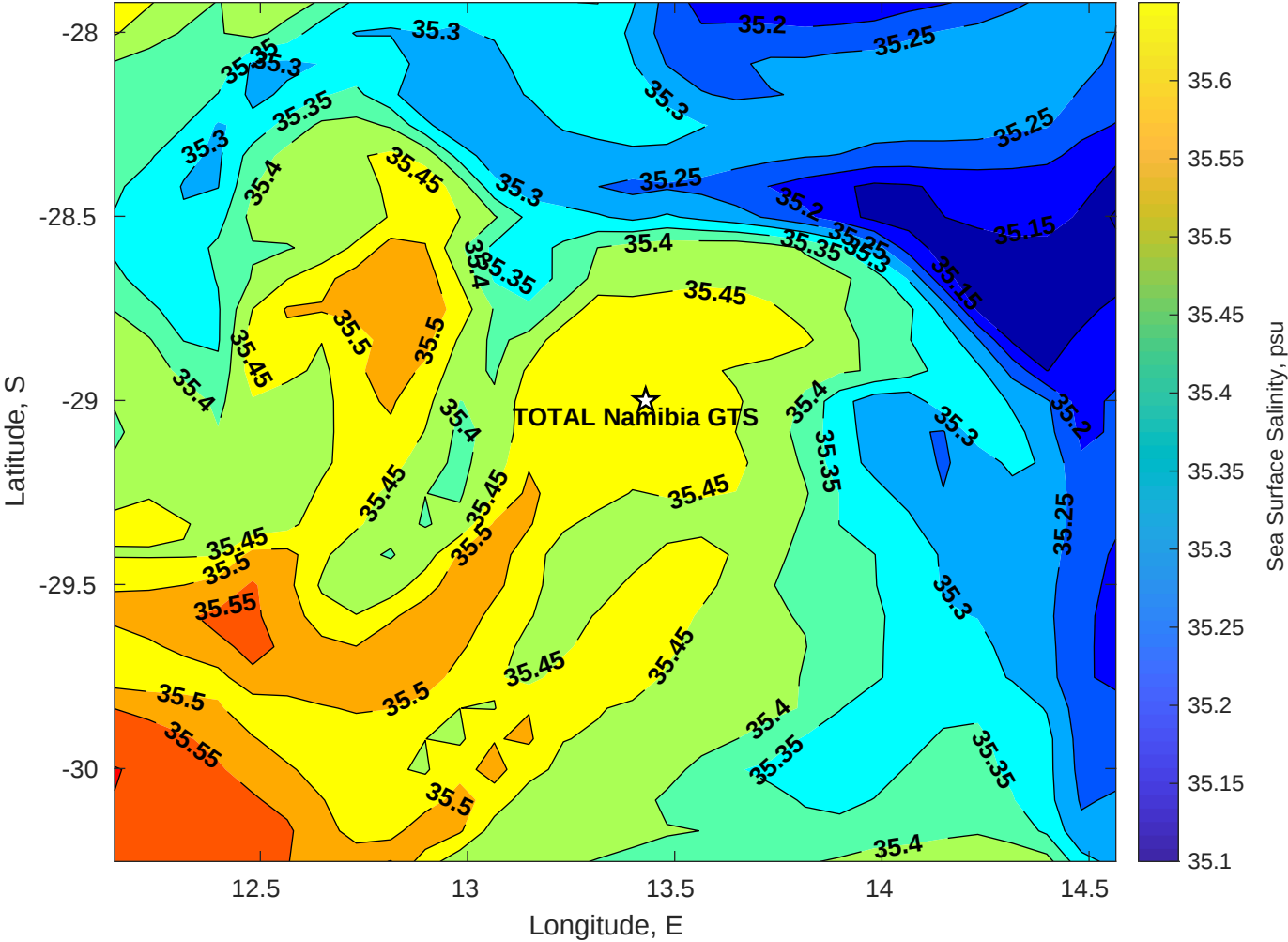
Surface Salinity for TOTAL Namibia GTS at 06-May-2025 00:00:00
