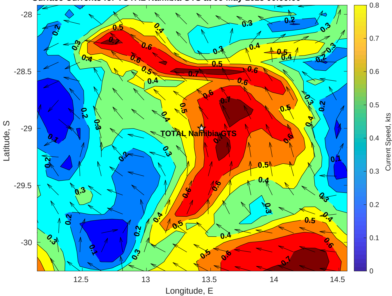
Surface Currents for TOTAL Namibia GTS at 06-May-2025 00:00:00
