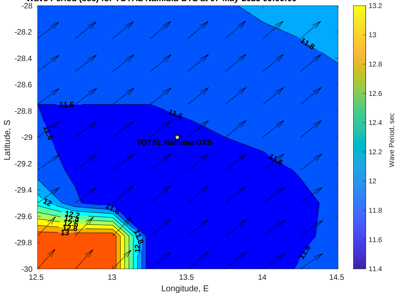
Wave Period (sec) for TOTAL Namibia GTS at 07-May-2025 09:00:00
