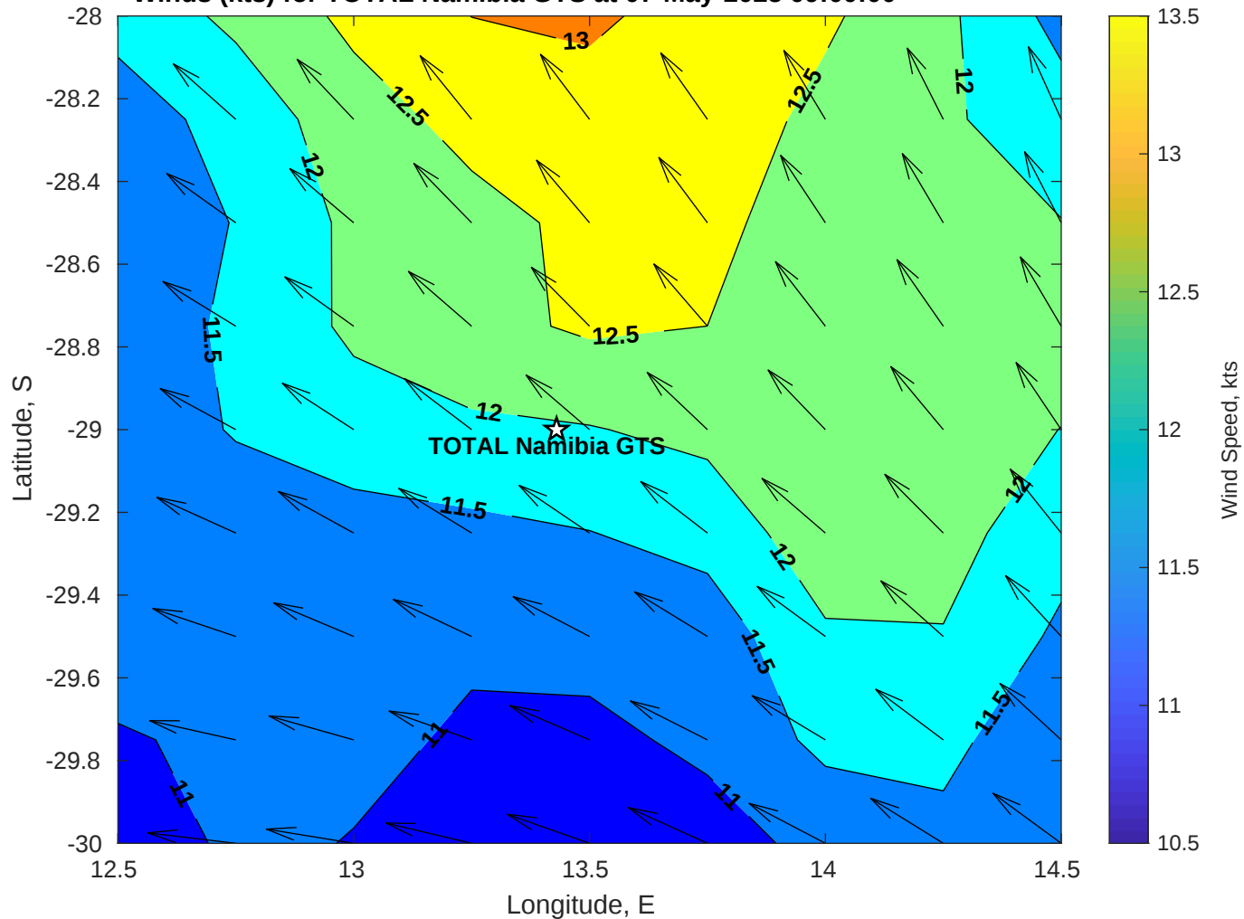
Winds (kts) for TOTAL Namibia GTS at 07-May-2025 09:00:00
