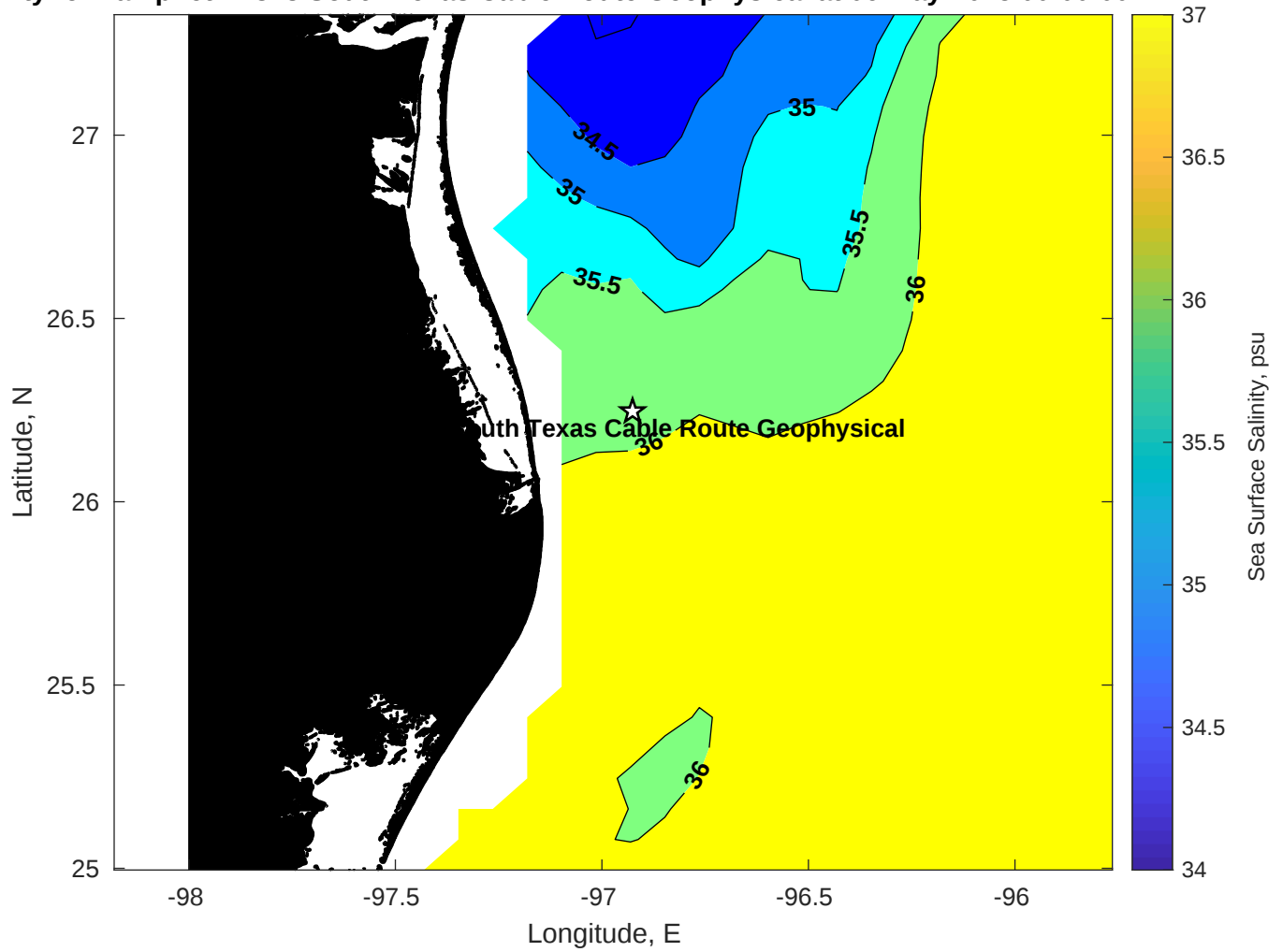
Surface Salinity for Tampnet P2378 South Texas Cable Route Geophysical at 06-May-2025 00:00:00
