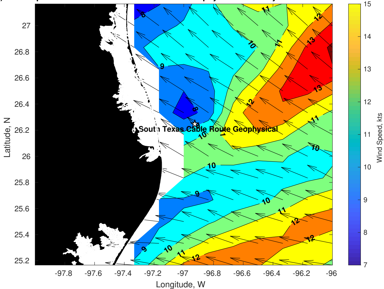
Winds (kts) for Tampnet P2378 South Texas Cable Route Geophysical at 07-May-2025 09:00:00
