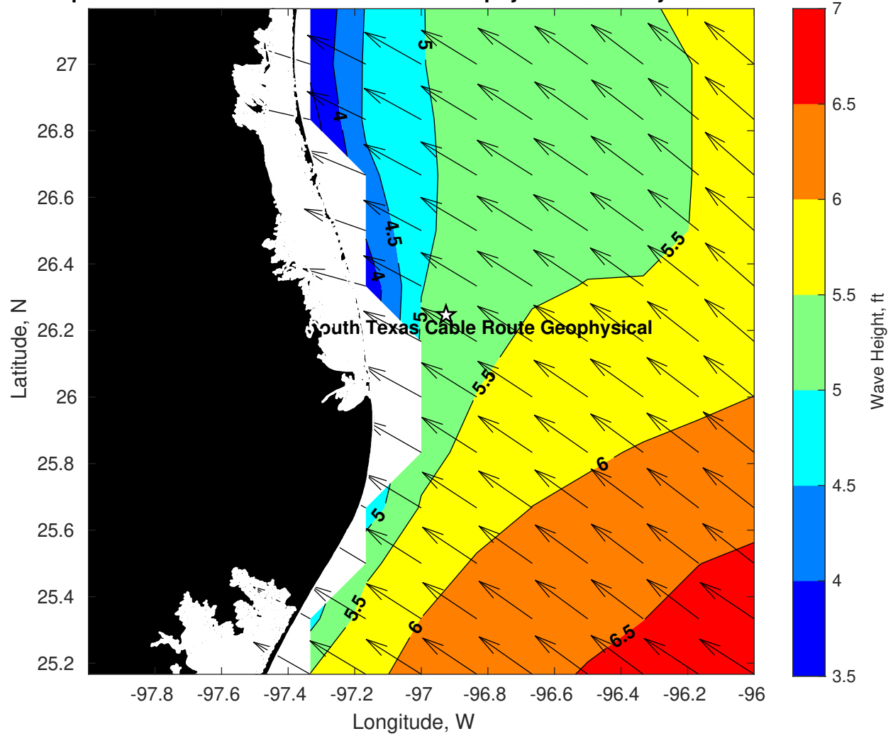
Wave Height (ft) for Tampnet P2378 South Texas Cable Route Geophysical at 07-May-2025 09:00:00
