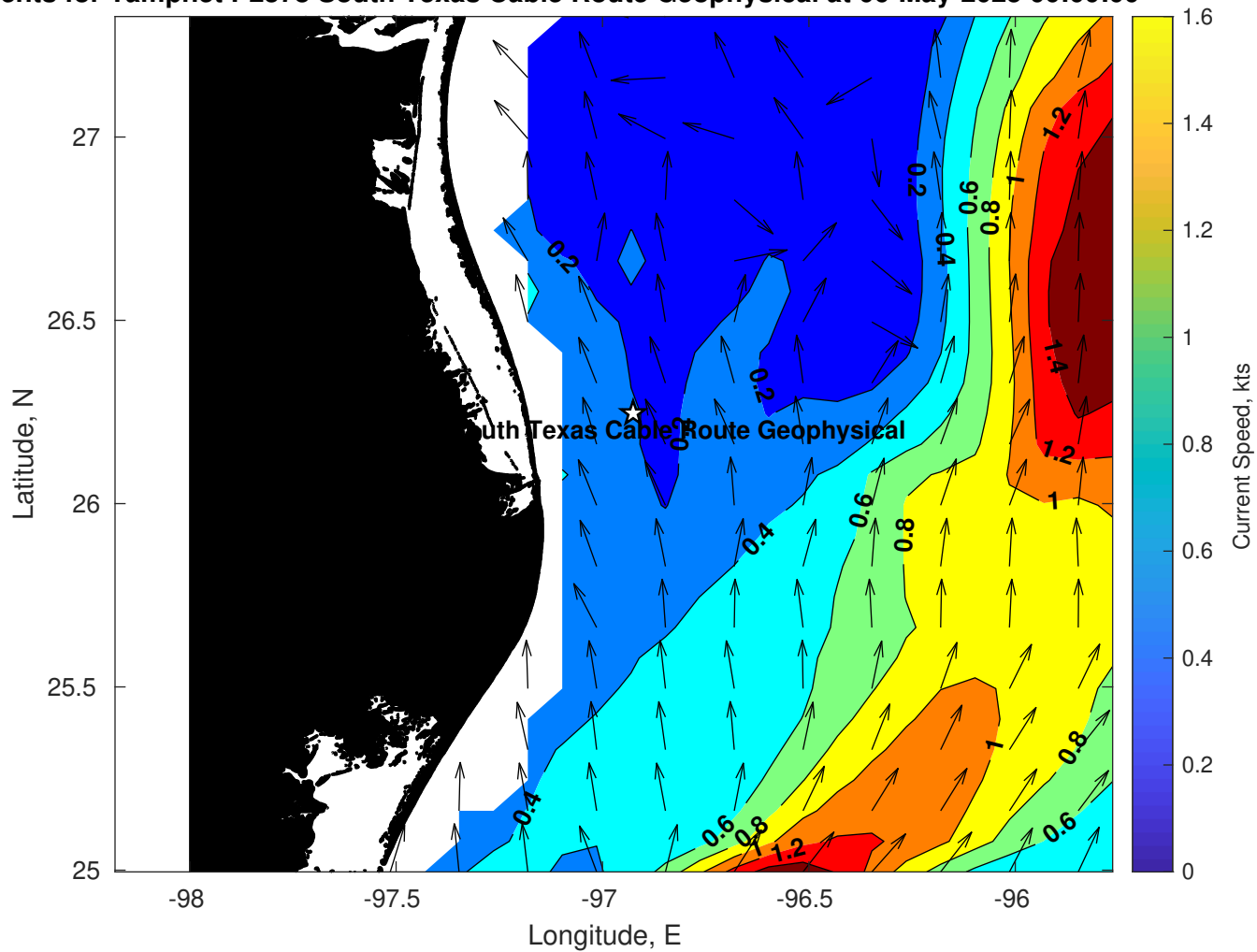
Surface Currents for Tampnet P2378 South Texas Cable Route Geophysical at 06-May-2025 00:00:00
