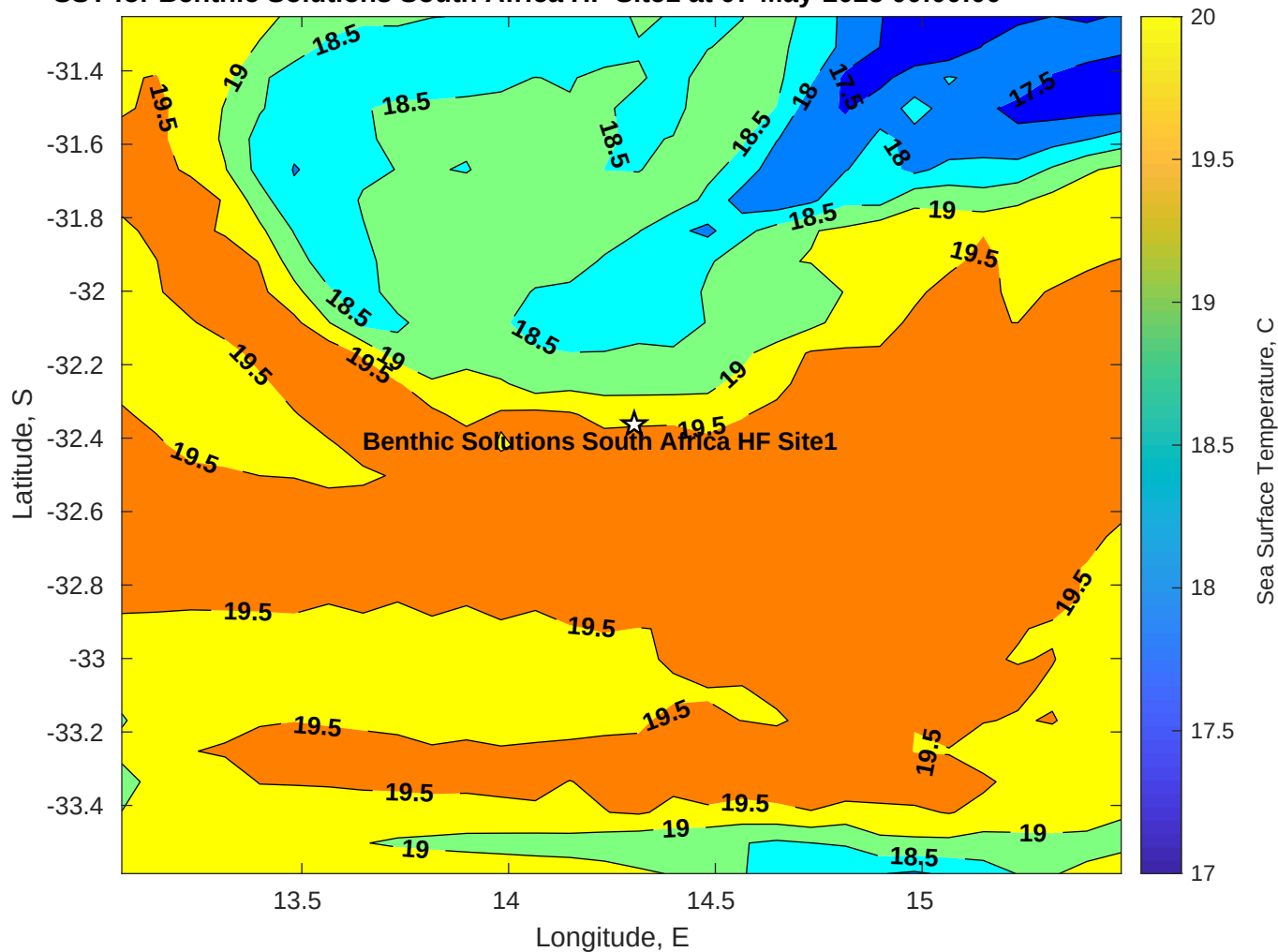
SST for Benthic Solutions South Africa HF Site1 at 07-May-2025 00:00:00
