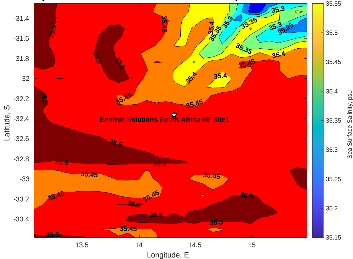
Surface Salinity for Benthic Solutions South Africa HF Site1 at 07-May-2025 00:00:00
