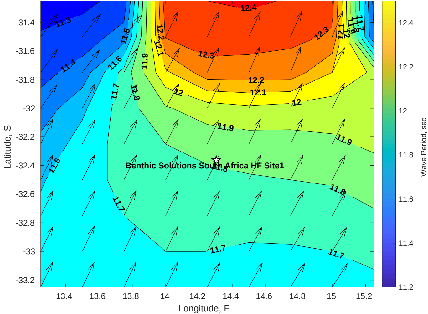
Wave Period (sec) for Benthic Solutions South Africa HF Site1 at 08-May-2025 09:00:00
