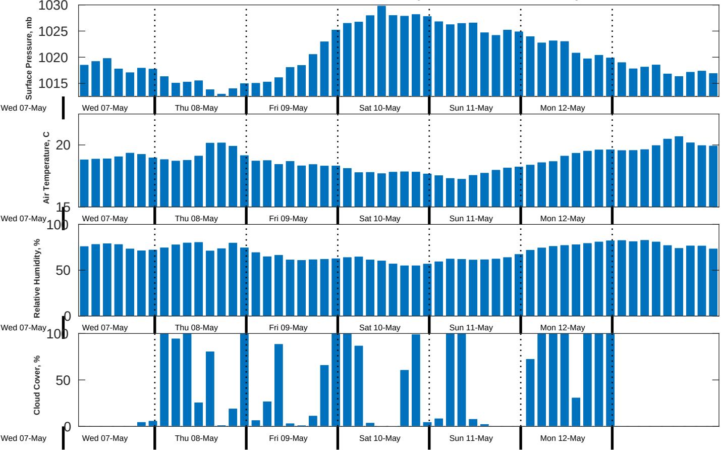
Met Forecast for Benthic Solutions South Africa HF Site1 from 08-May-2025 00:00:00 to 15-May-2025 00:00:00
