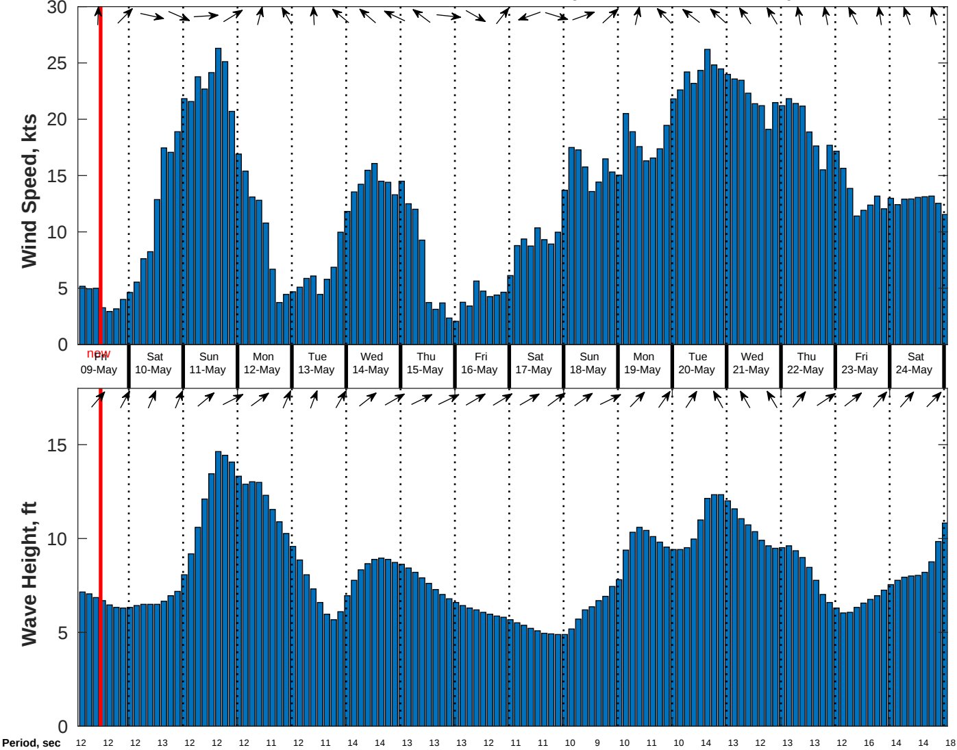
Wind & Wave Forecast for Benthic Solutions South Africa HF Site2 from 08-May-2025 02:00:00 to 24-May-2025 02:00:00
