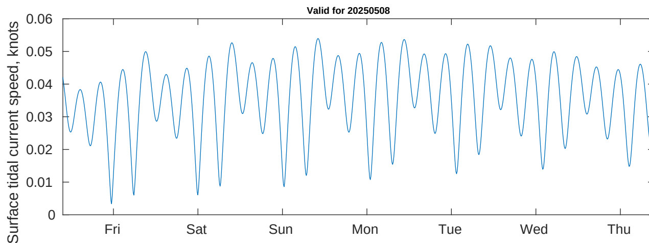
Tidal Currents and Heights for Benthic Solutions South Africa HF Site3 at 20250508
