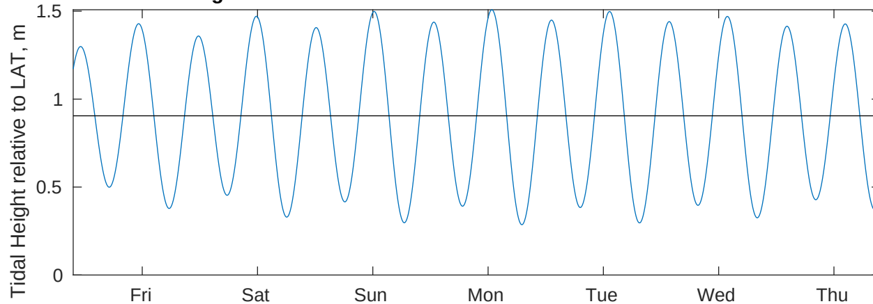
Tidal Currents and Heights for Benthic Solutions South Africa HF Site3 at 20250508
