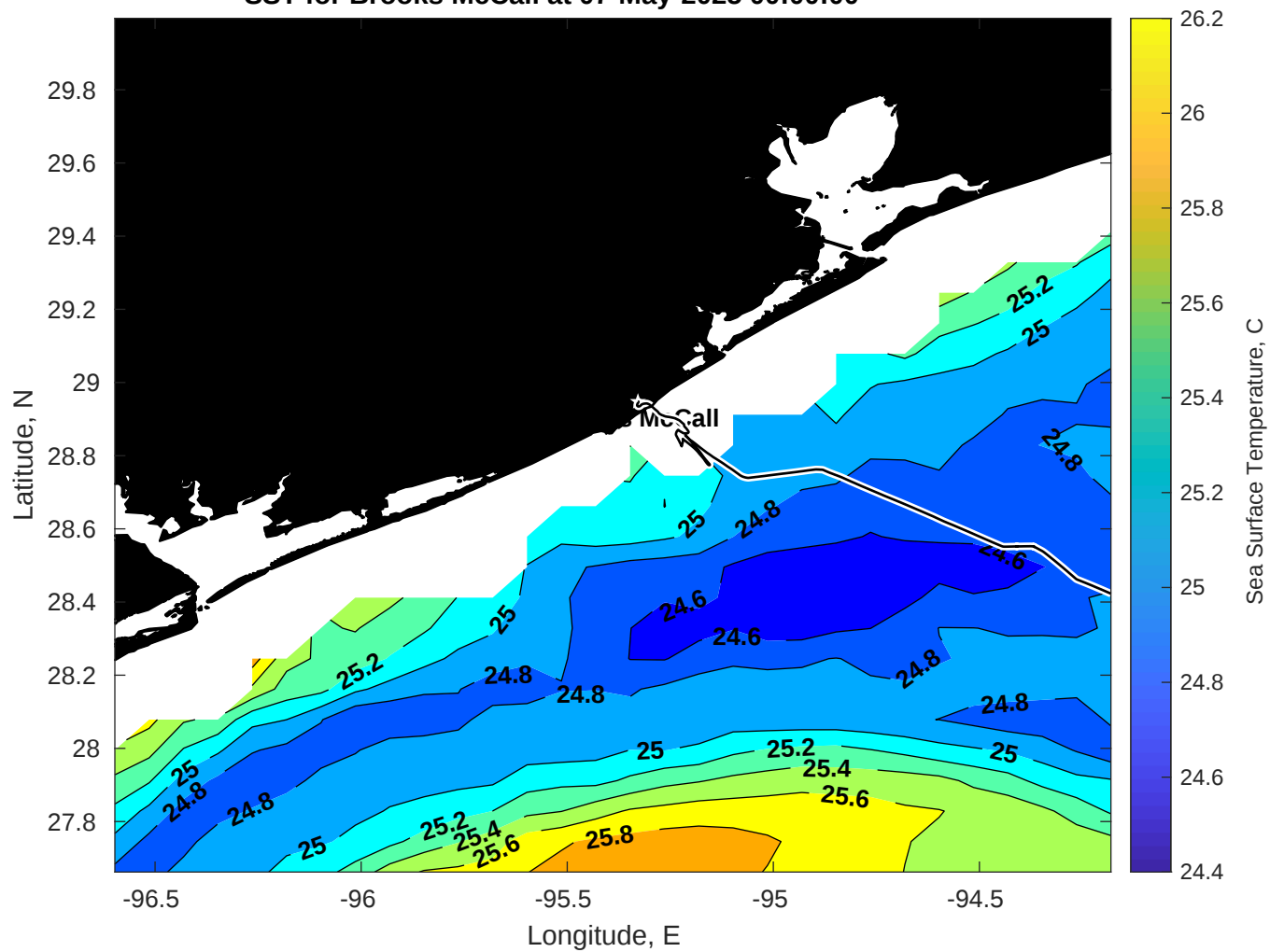
SST for Brooks McCall at 07-May-2025 00:00:00
