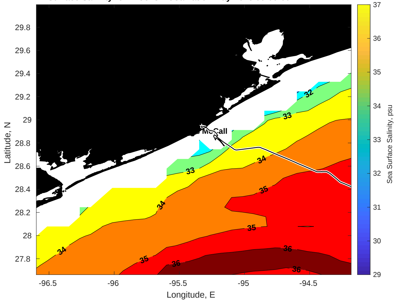
Surface Salinity for Brooks McCall at 07-May-2025 00:00:00
