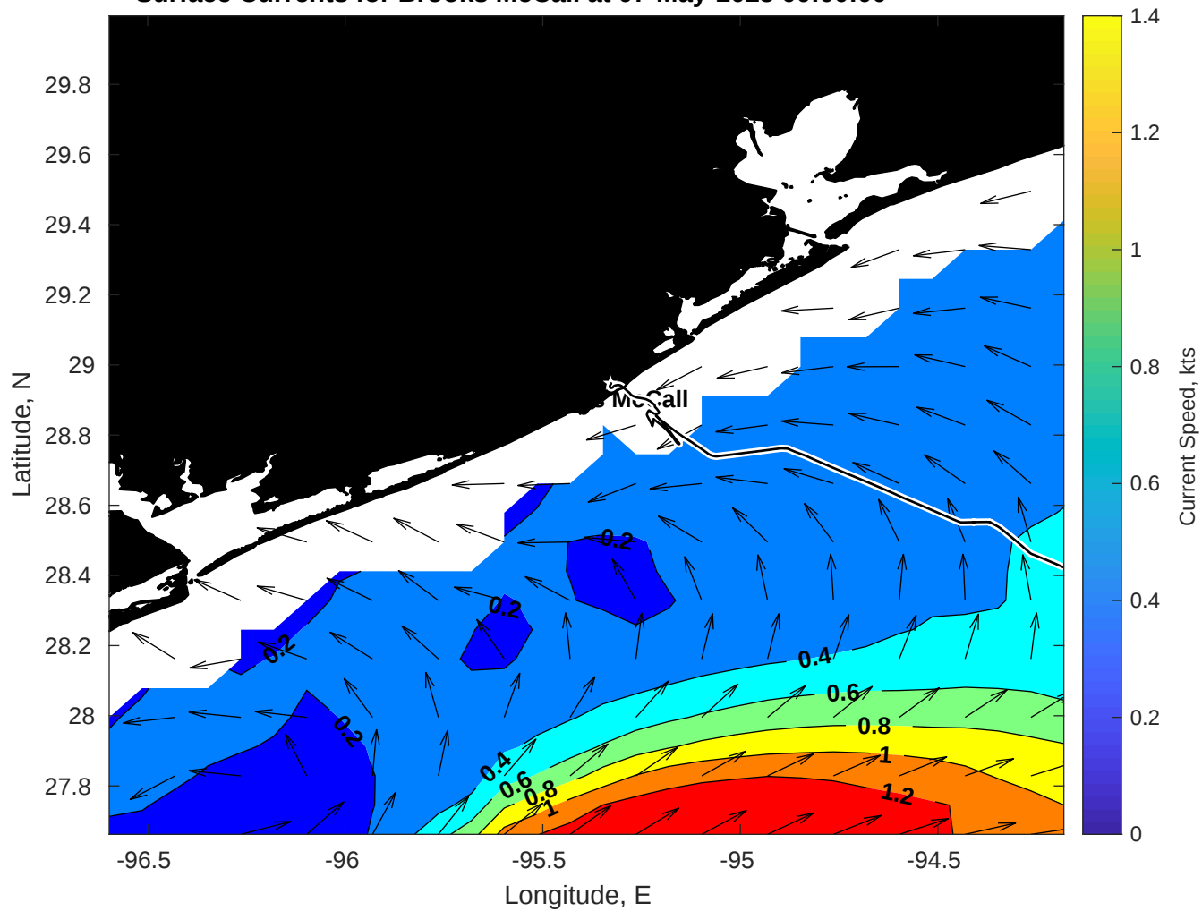
Surface Currents for Brooks McCall at 07-May-2025 00:00:00
