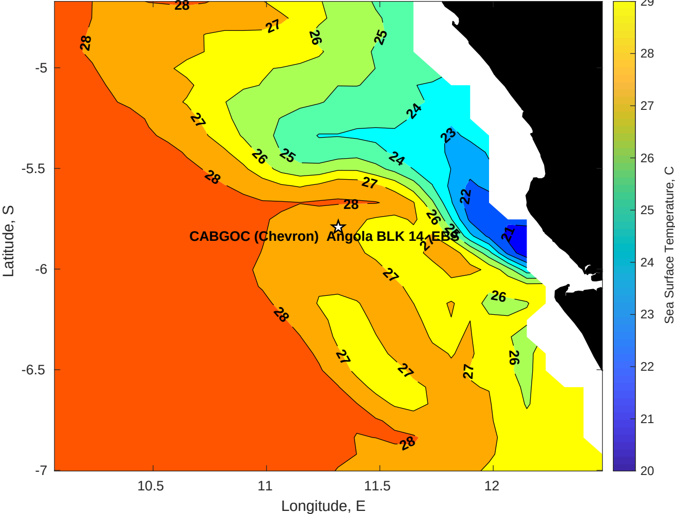
SST for CABGOC (Chevron) Angola BLK 14 EBS at 07-May-2025 00:00:00
