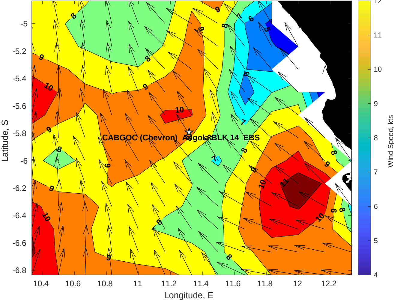
Winds (kts) for CABGOC (Chevron) Angola BLK 14 EBS at 08-May-2025 09:00:00
