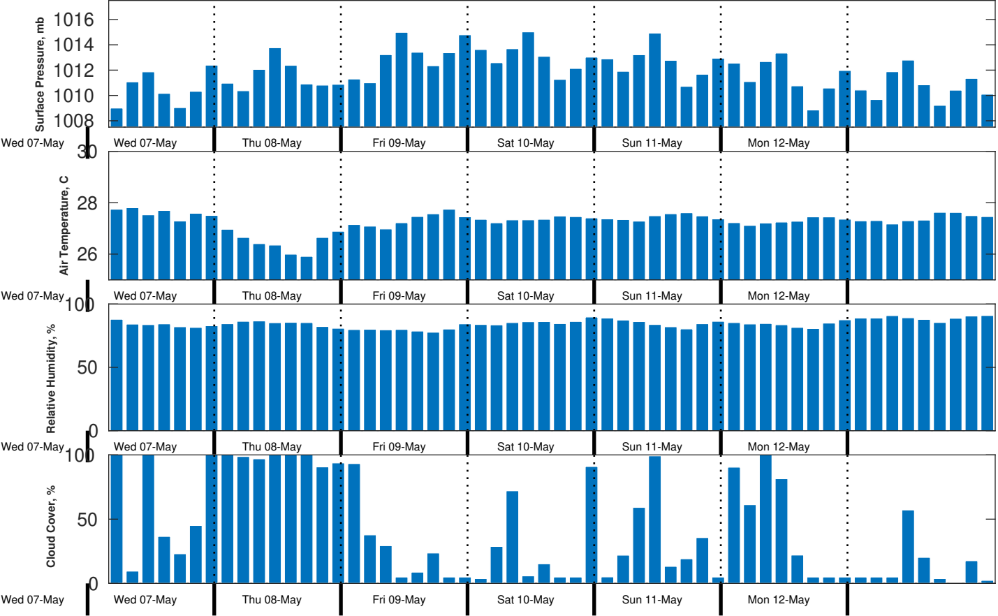
Met Forecast for CABGOC (Chevron) Angola BLK 14 EBS from 08-May-2025 00:00:00 to 15-May-2025 00:00:00
