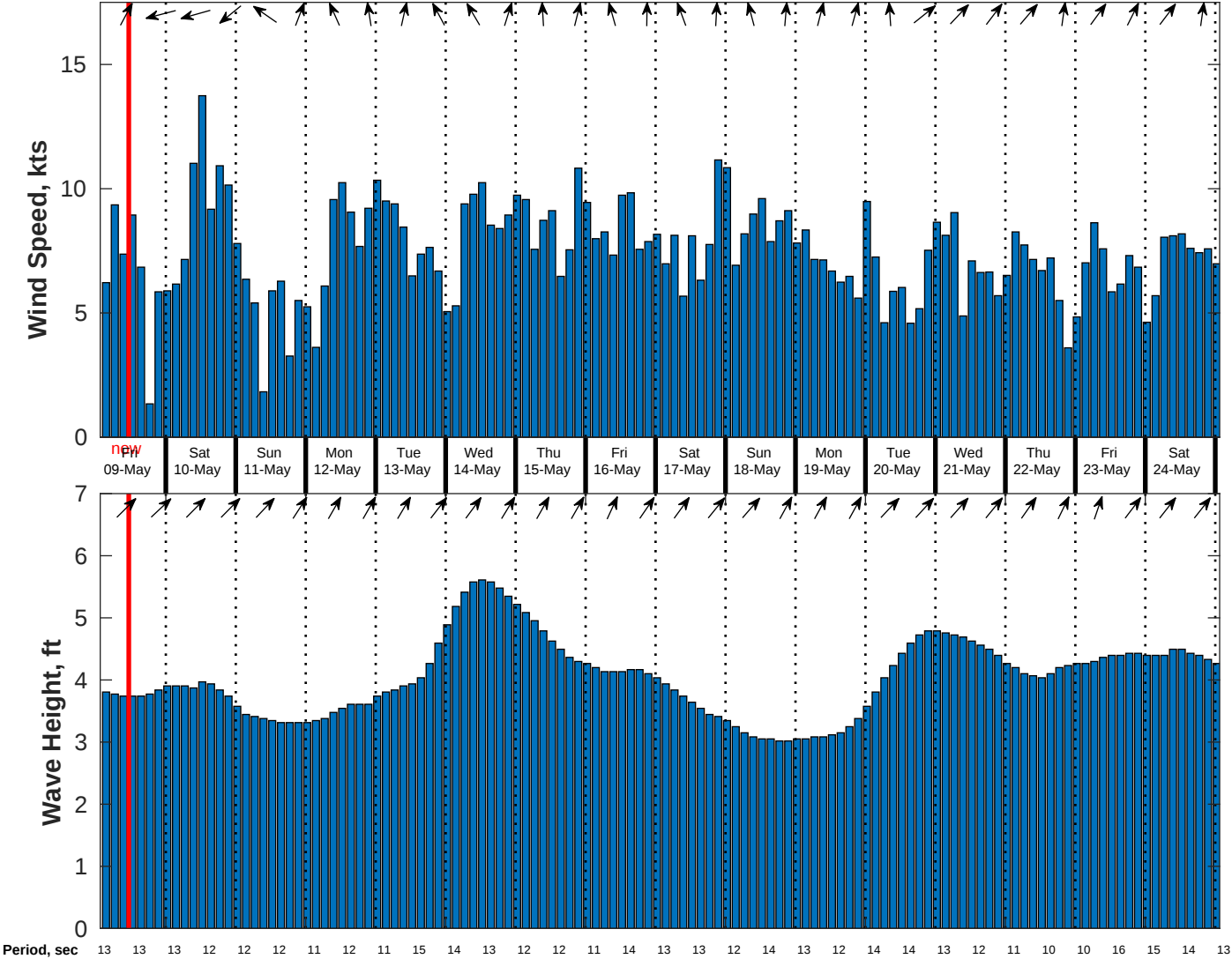
Wind & Wave Forecast for CABGOC (Chevron) Angola BLK 14 EBS from 08-May-2025 02:00:00 to 24-May-2025 02:00:00
