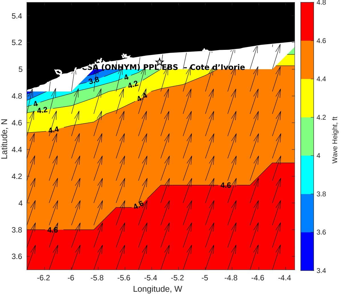
Wave Height (ft) for CSA (ONHYM) PPL EBS - Cote d'Ivoire at 08-May-2025 09:00:00
