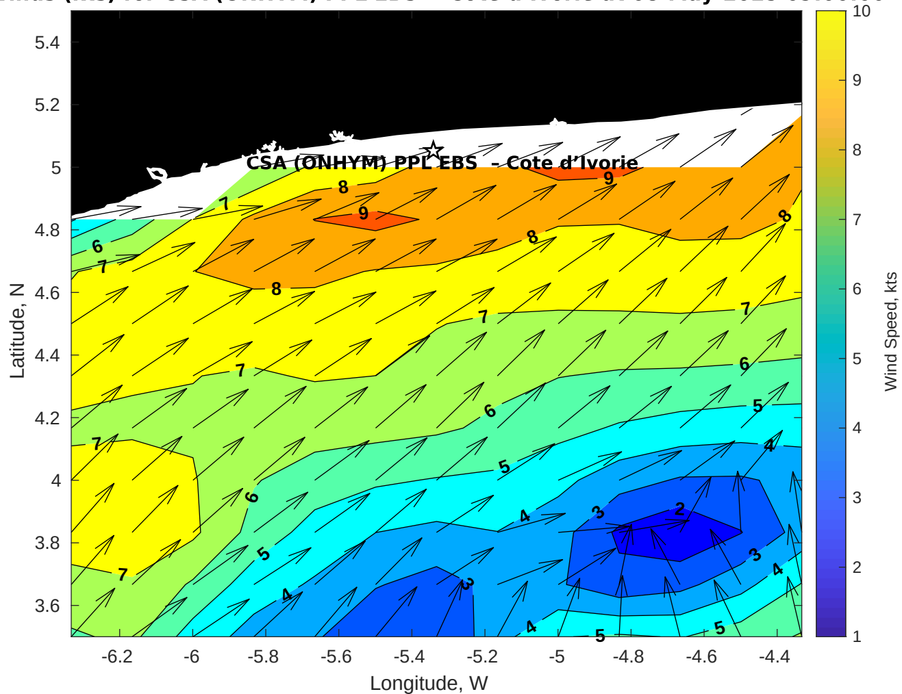
Winds (kts) for CSA (ONHYM) PPL EBS - Cote d'Ivoire at 08-May-2025 09:00:00
