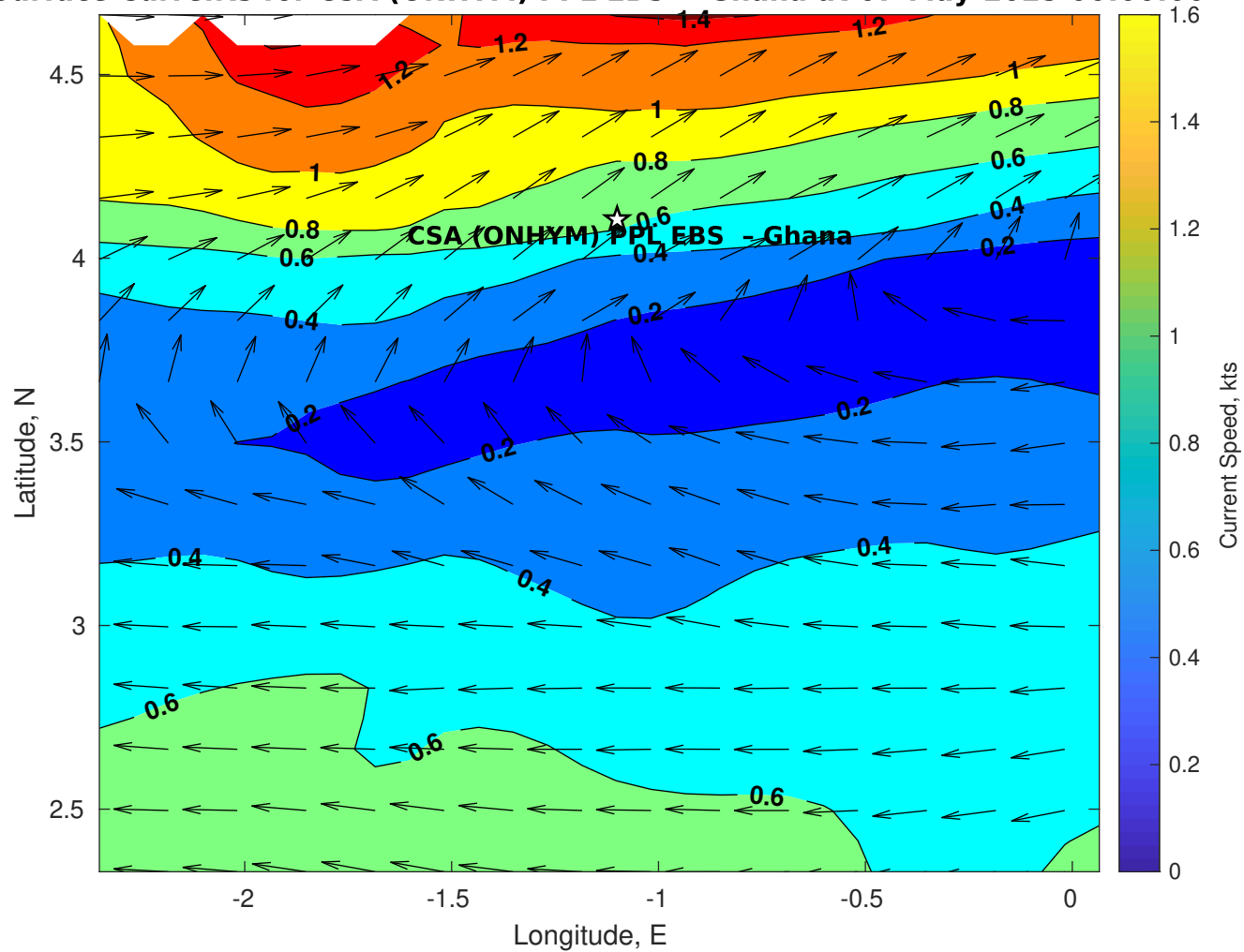
Surface Currents for CSA (ONHYM) PPL EBS - Ghana at 07-May-2025 00:00:00
