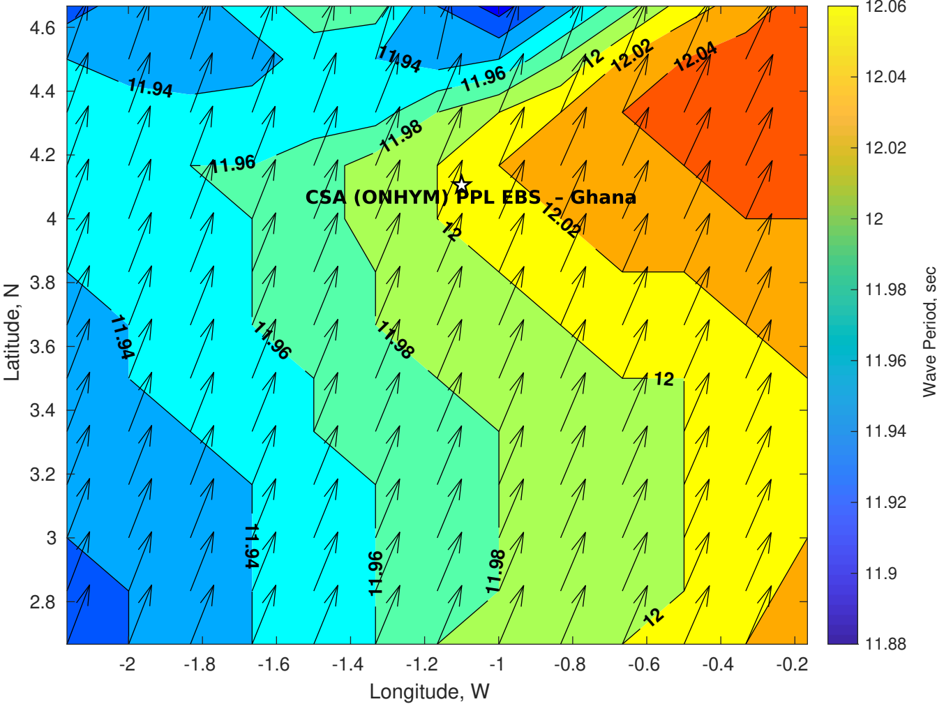
Wave Period (sec) for CSA (ONHYM) PPL EBS - Ghana at 08-May-2025 09:00:00
