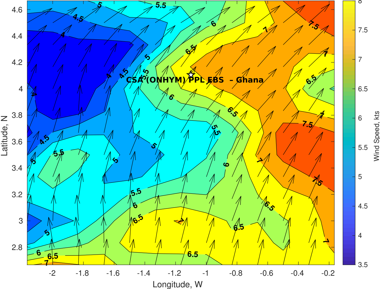
Winds (kts) for CSA (ONHYM) PPL EBS - Ghana at 08-May-2025 09:00:00
