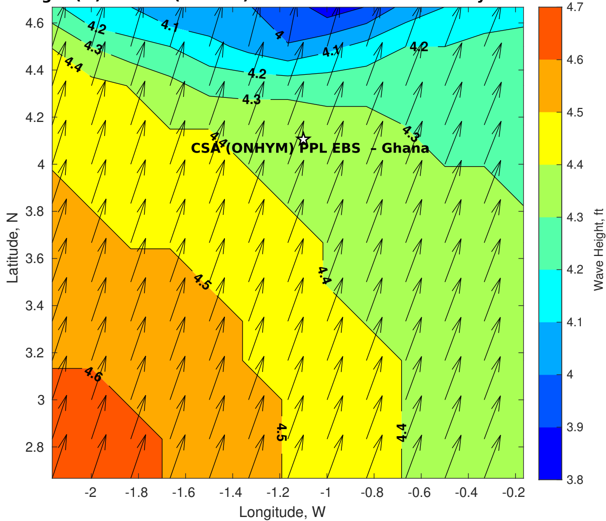
Wave Height (ft) for CSA (ONHYM) PPL EBS - Ghana at 08-May-2025 09:00:00
