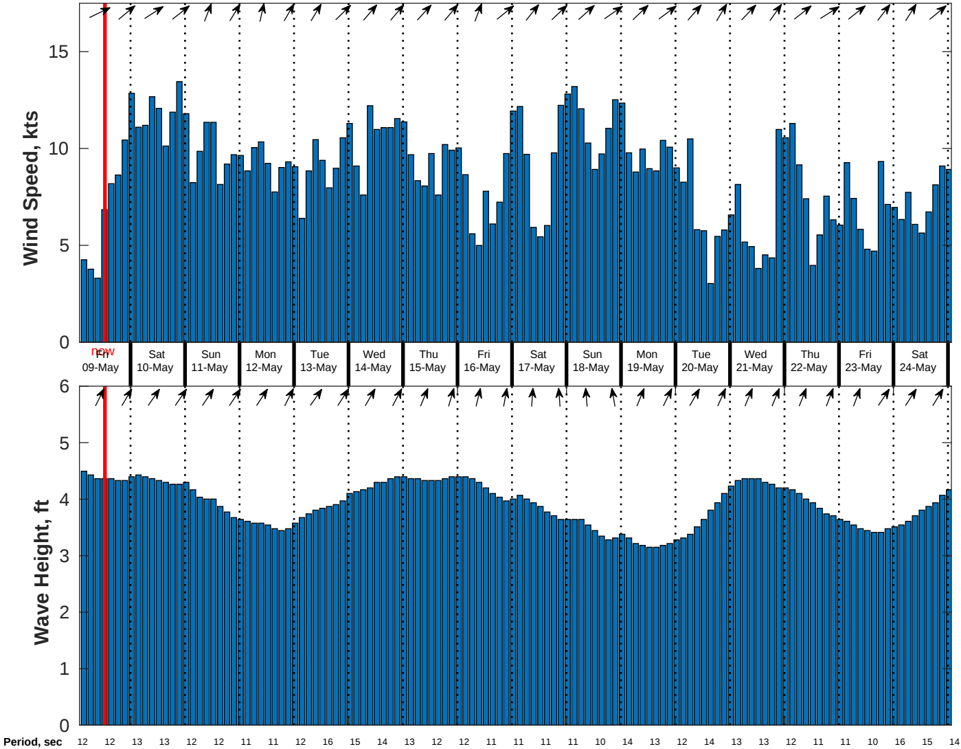
Wind & Wave Forecast for CSA (ONHYM) PPL EBS - Ghana from 08-May-2025 02:00:00 to 24-May-2025 02:00:00
