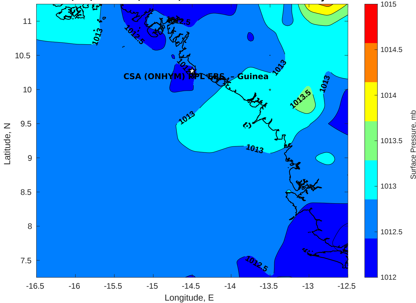
Surface Pressure (mb) for CSA (ONHYM) PPL EBS - Guinea at 09-May-2025 00:00:00
