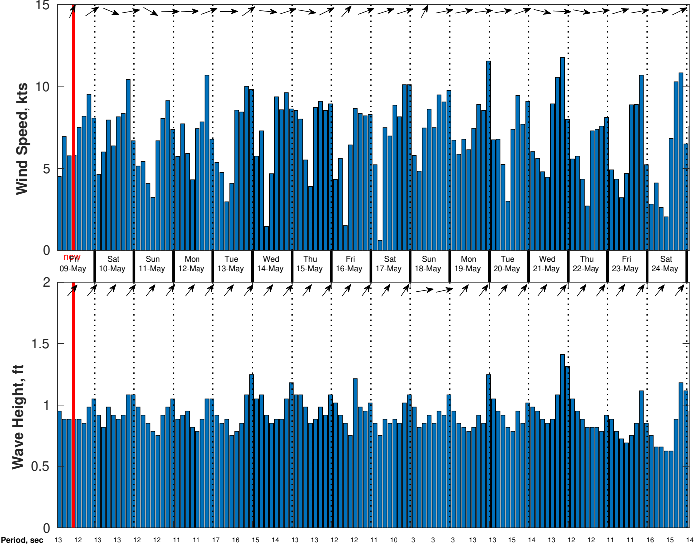
Wind & Wave Forecast for CSA (ONHYM) PPL EBS - Guinea from 08-May-2025 01:00:00 to 24-May-2025 01:00:00
