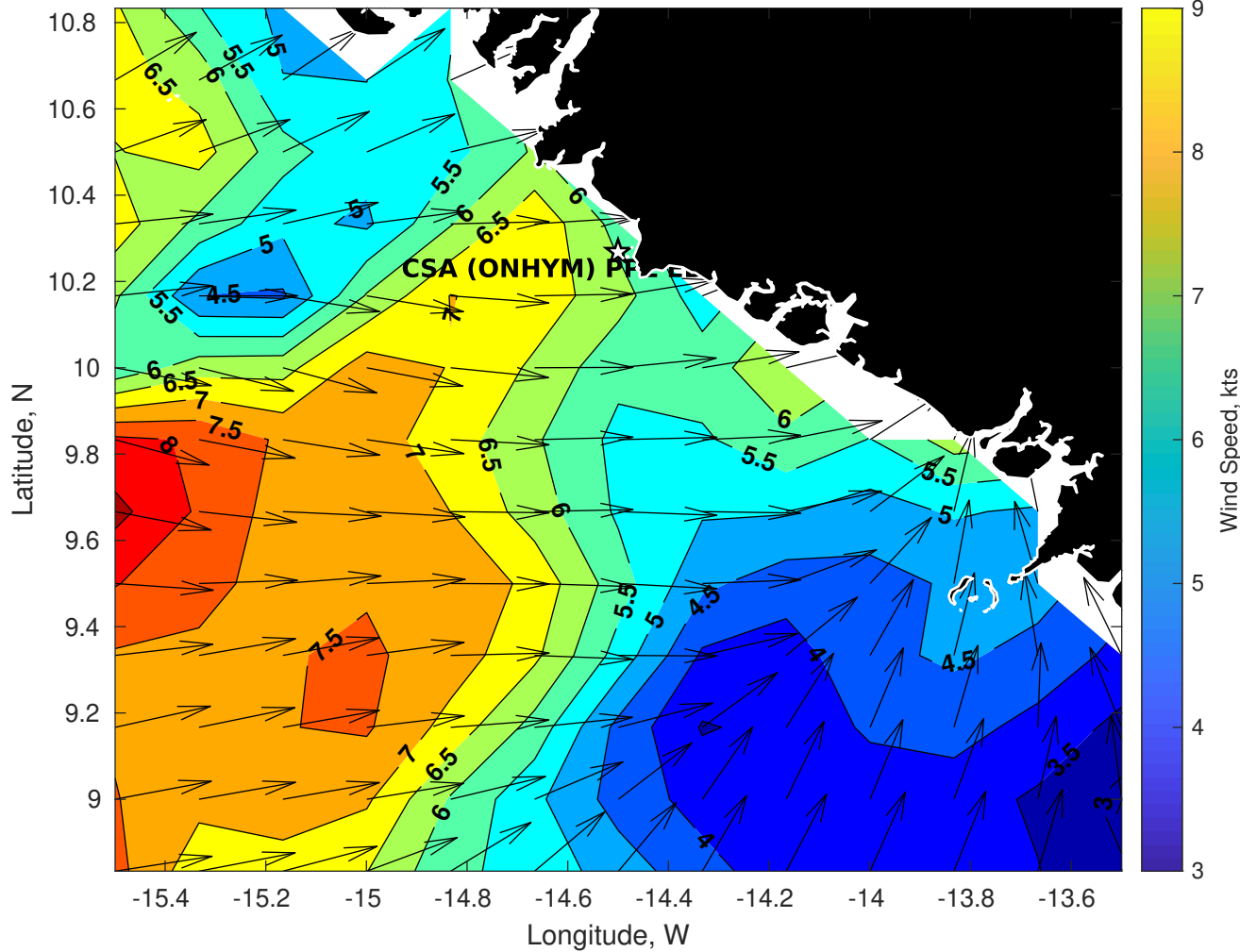
Winds (kts) for CSA (ONHYM) PPL EBS - Guinea at 08-May-2025 09:00:00
