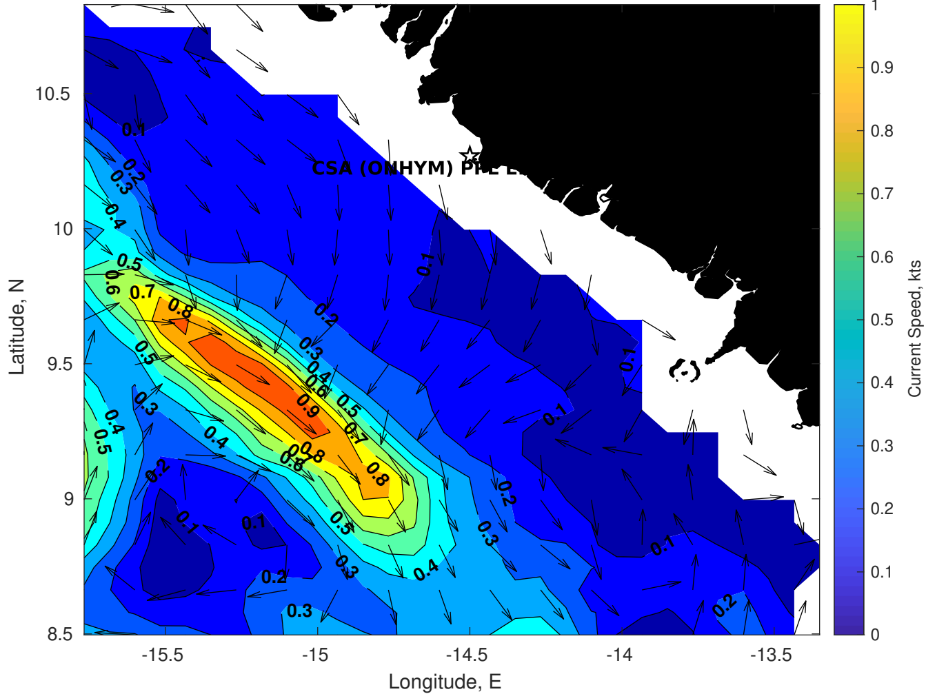
Surface Currents for CSA (ONHYM) PPL EBS - Guinea at 07-May-2025 00:00:00
