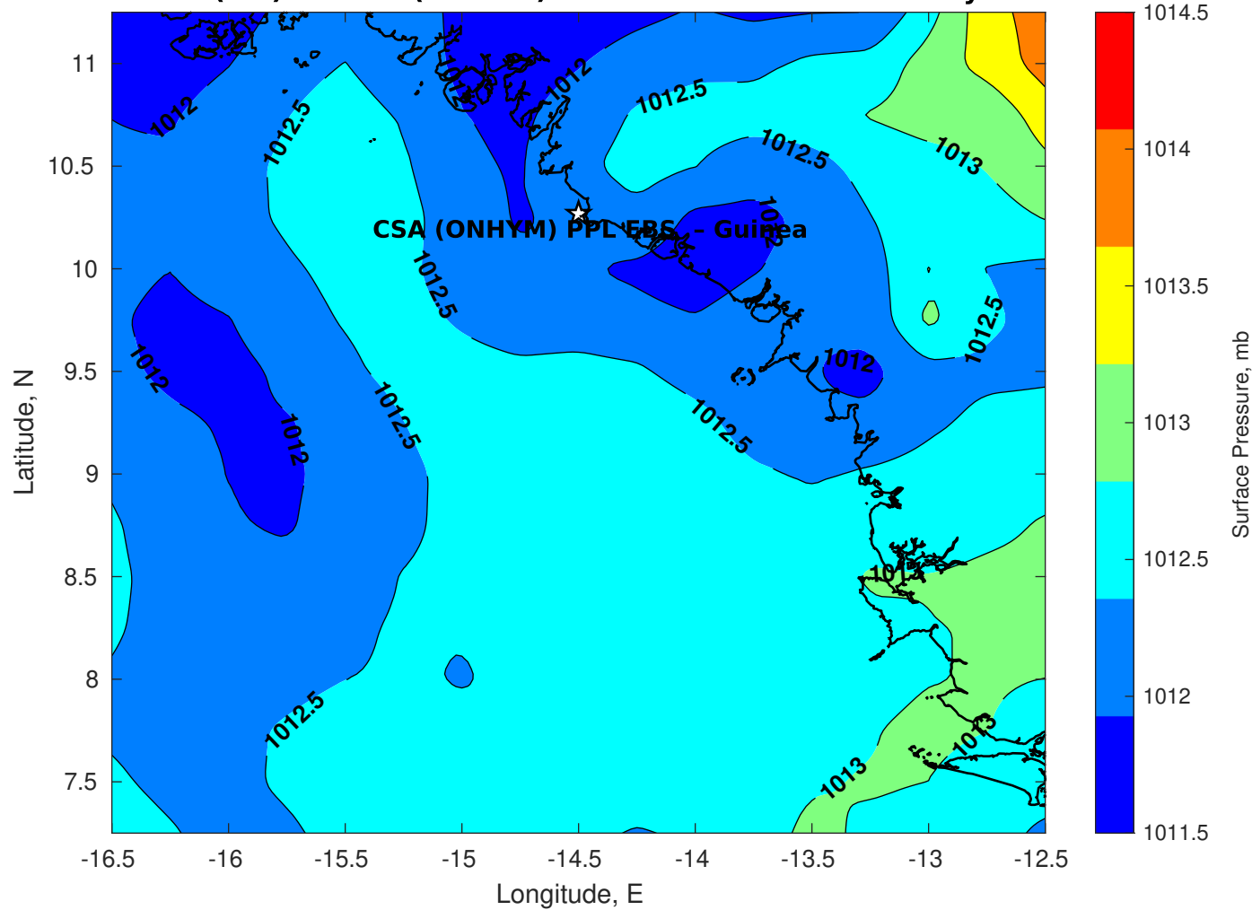
Surface Pressure (mb) for CSA (ONHYM) PPL EBS - Guinea at 08-May-2025 00:00:00
