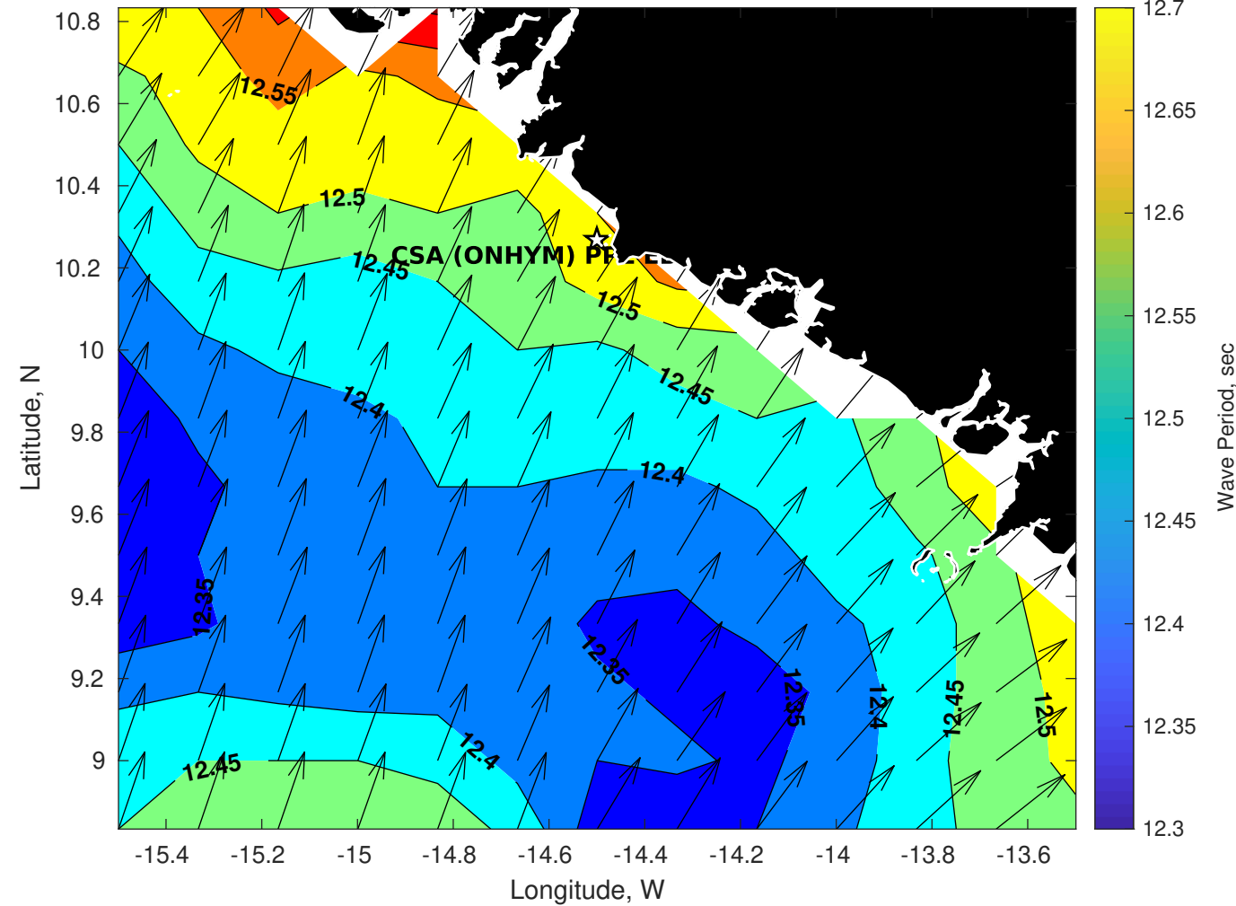
Wave Period (sec) for CSA (ONHYM) PPL EBS - Guinea at 08-May-2025 09:00:00
