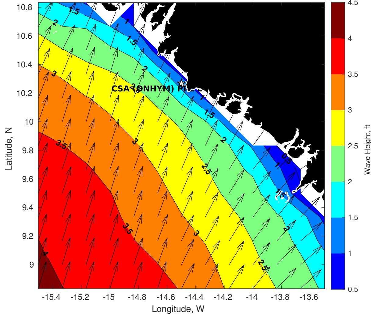
Wave Height (ft) for CSA (ONHYM) PPL EBS - Guinea at 08-May-2025 09:00:00
